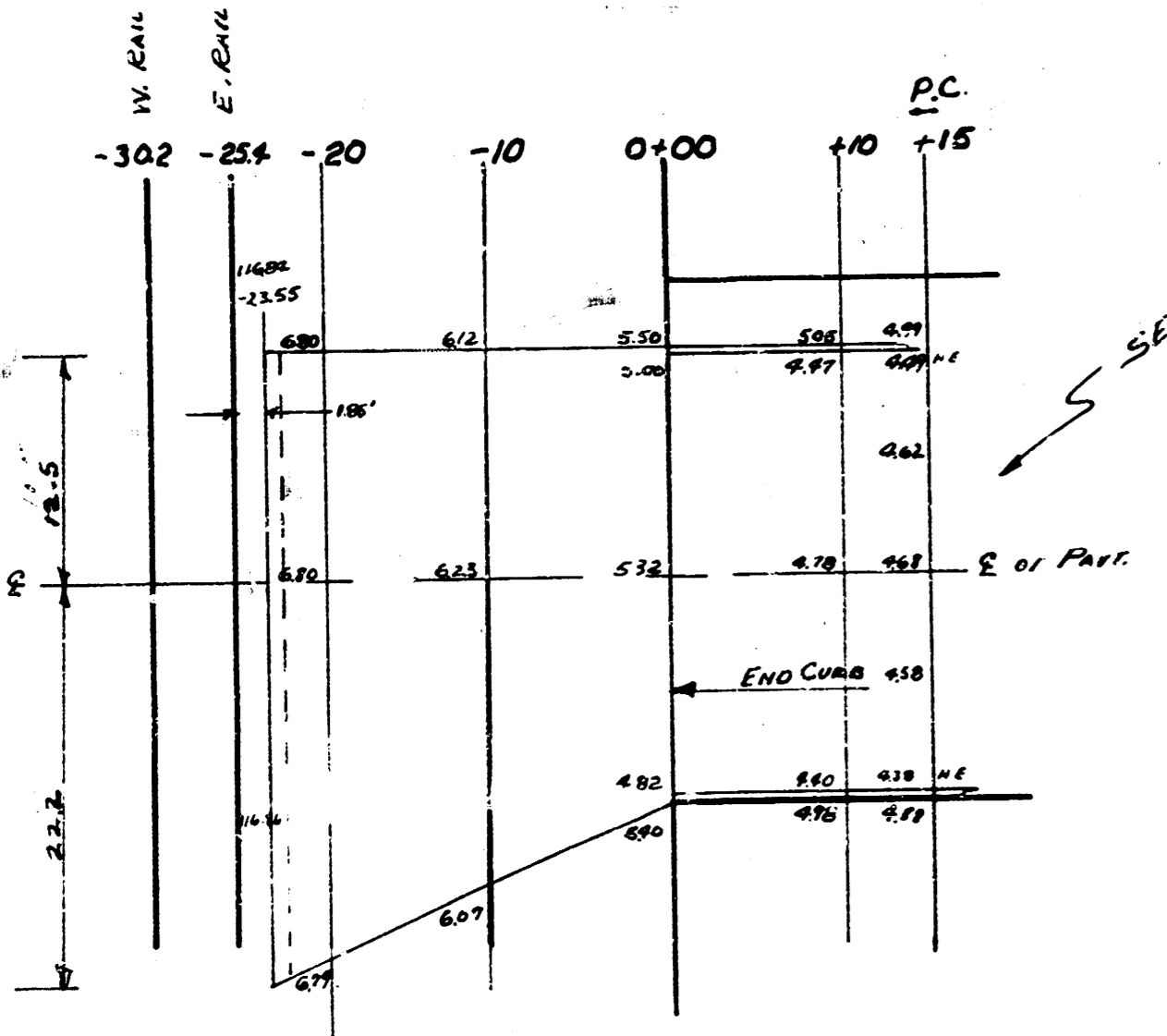
ELEV. DETAIL - R.R. CROSSING E 1/2
