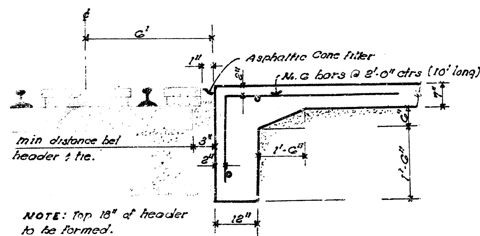
R. ROAD CROSSING DETAIL - 12" Scale -
