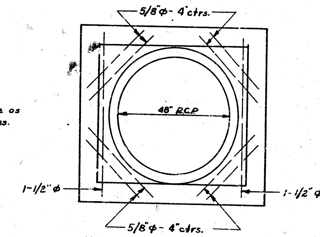
SECTION Showing steel pattern around 48" pipe.
