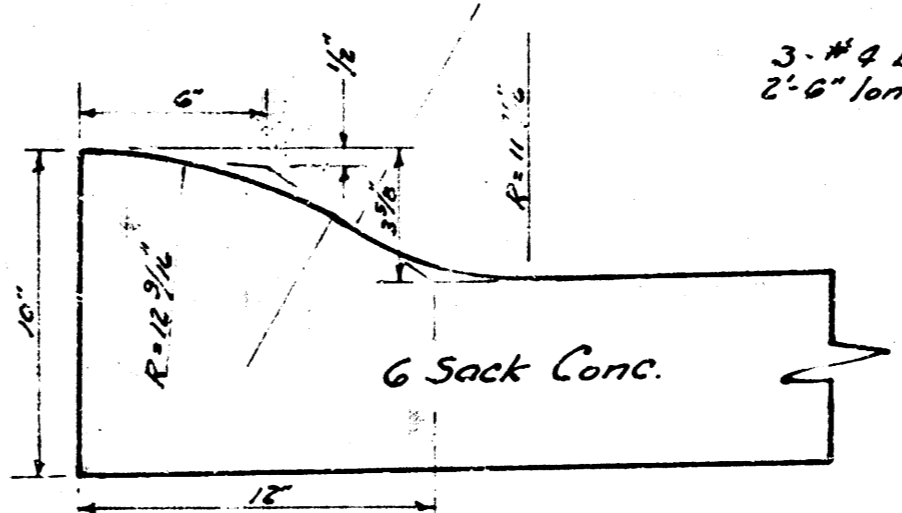
ROLL CURB DETAIL No Scale
