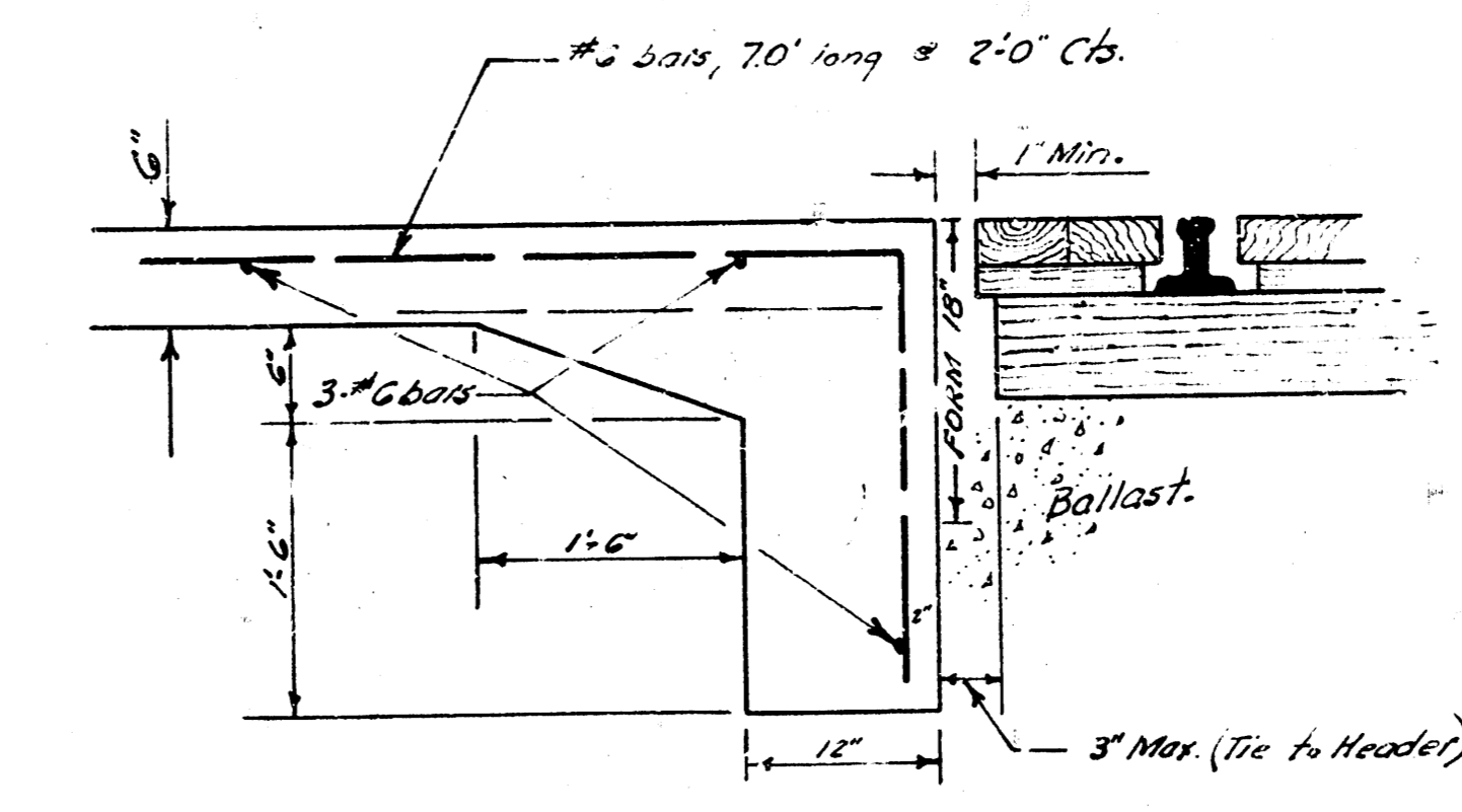
CONC. HEADER DETAIL FOR R.R. CROSSINGS No Scale
