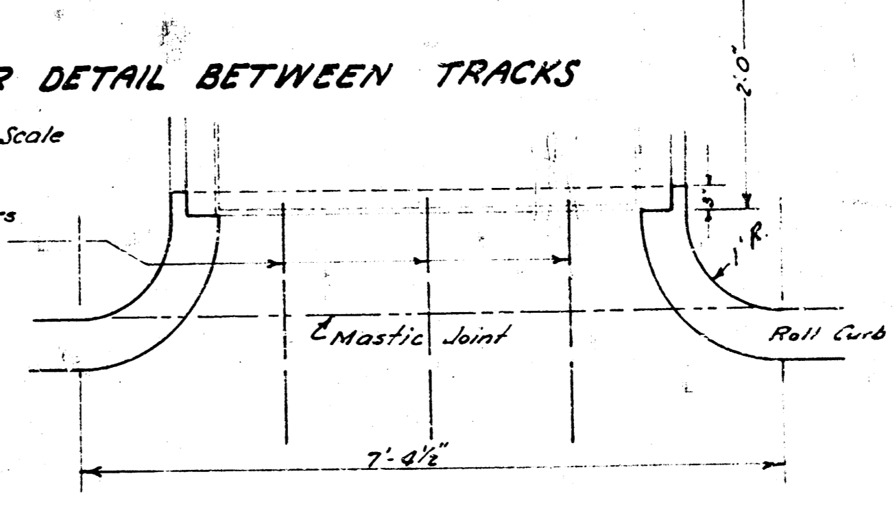
PLAN VIEW OF SETBACK FOR 2'x5' INLET No Scale
