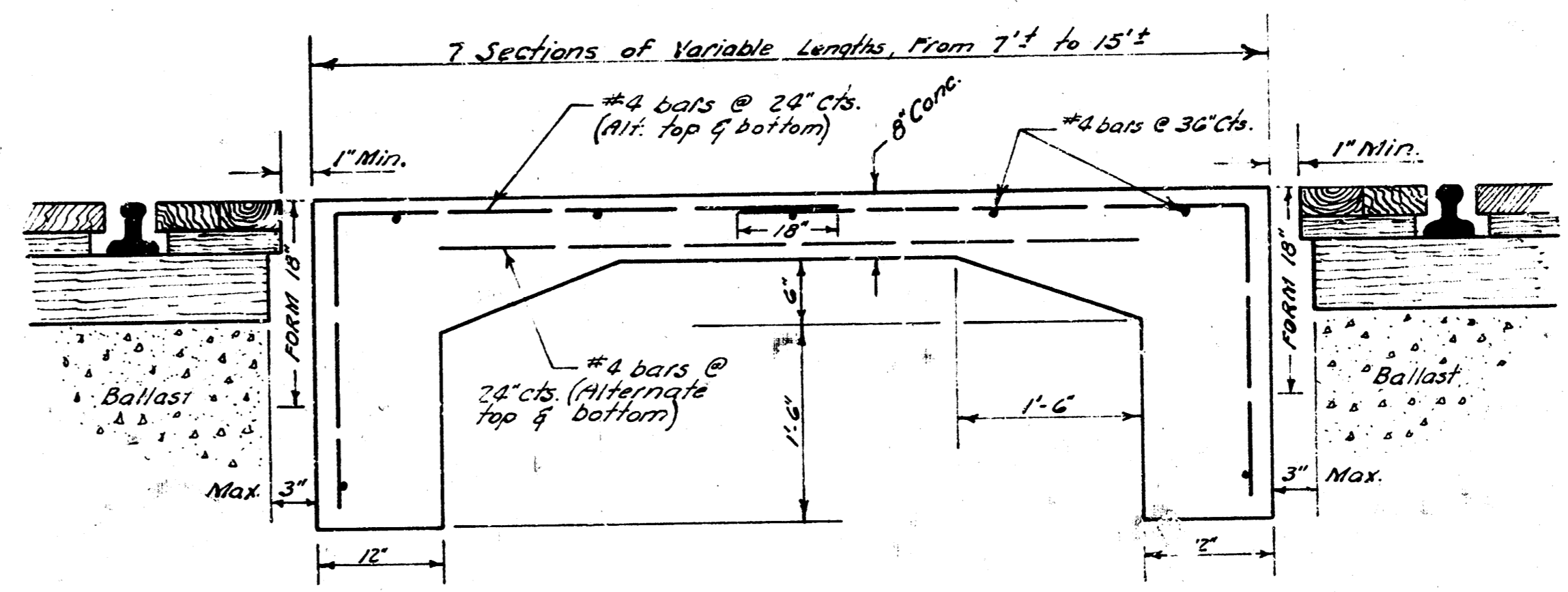
CONC. PAVEMENT & HEADER DETAIL BETWEEN TRACKS No Scale
