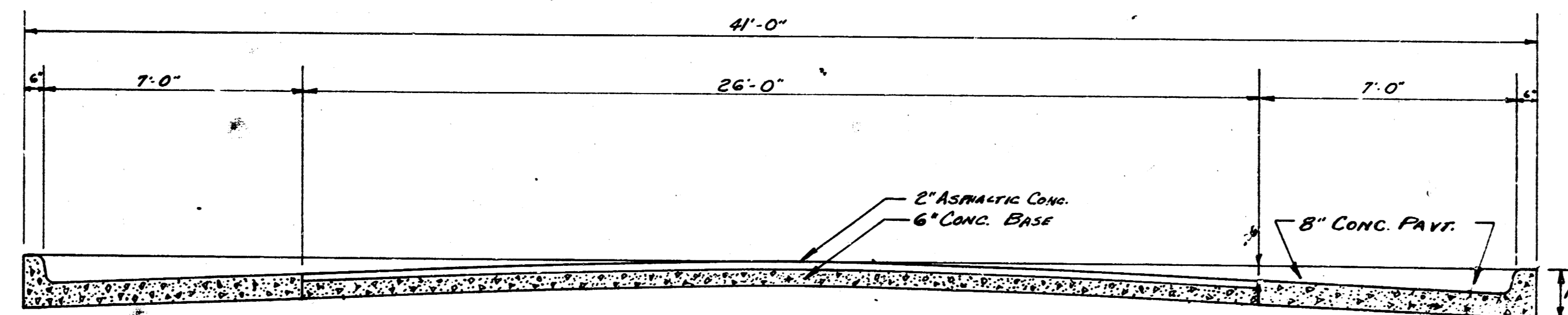
TYPICAL SECTION
