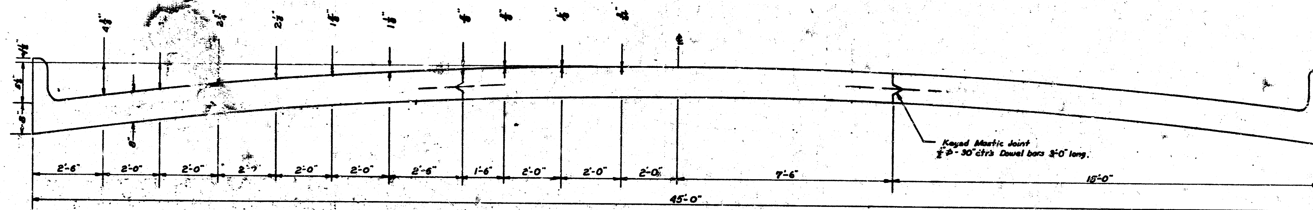
TYPICAL SECTION
