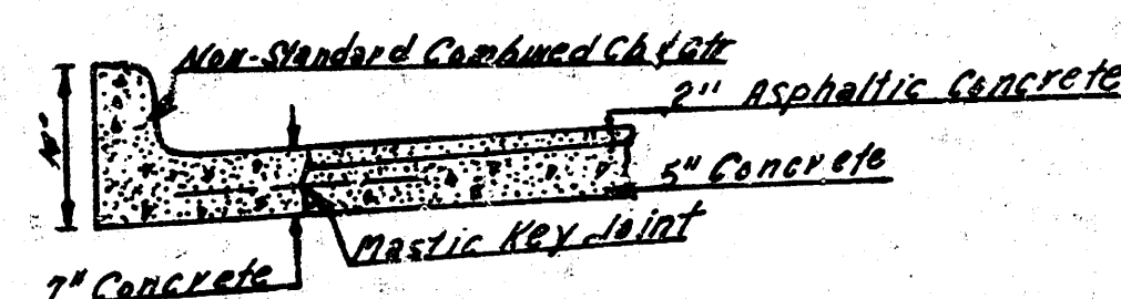
DETAIL OF NON-STANDARD COMB. CURB & GTR NO SCALE
