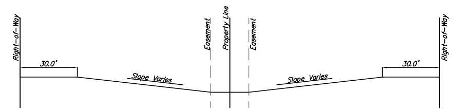
Typical Lot Grading Section
