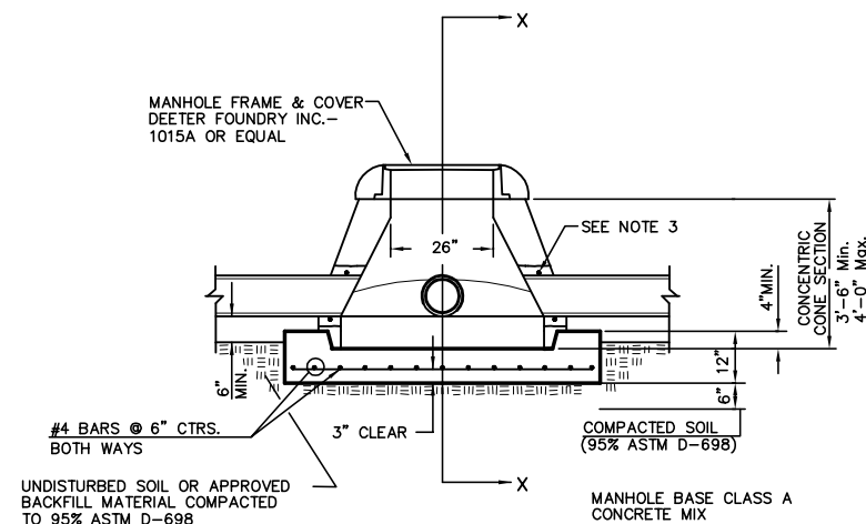
SPECIAL SHALLOW TYPE "P" MANHOLE
