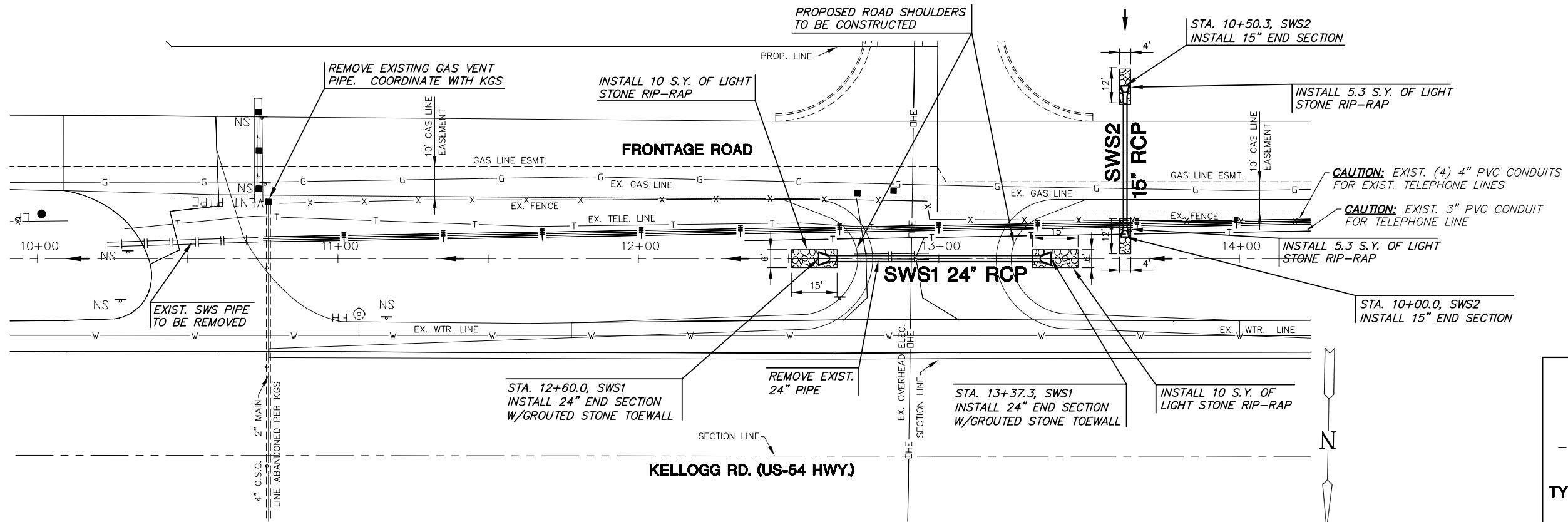
PLAN SWS1 SCALE: 1"=20'
