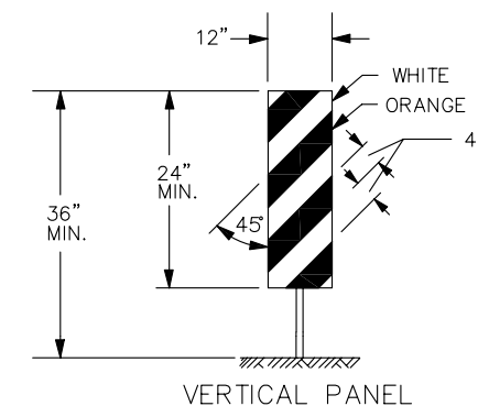
VERTICAL PANEL
