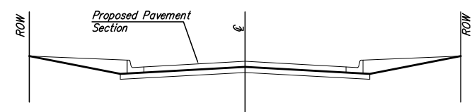
ROW GRADING DETAIL
