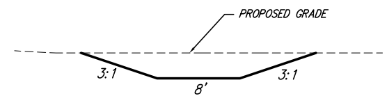
TEMPORARY DITCH DETAIL
