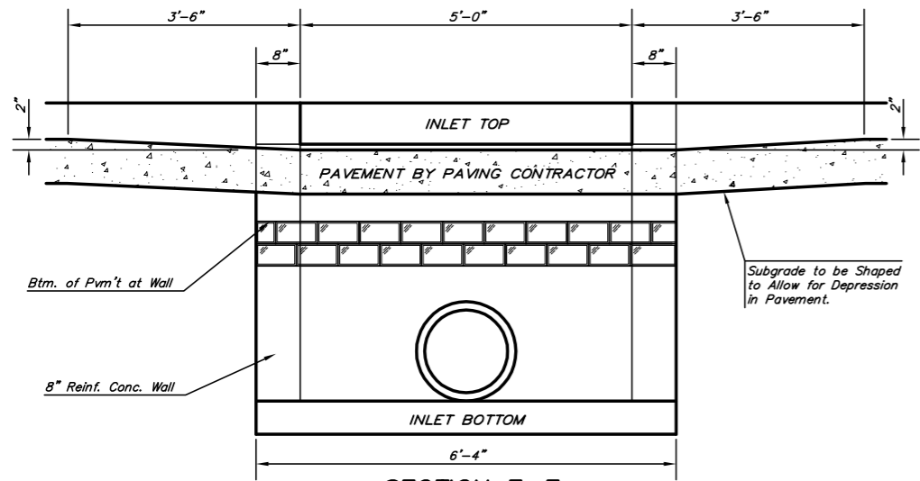
SECTION E-E
