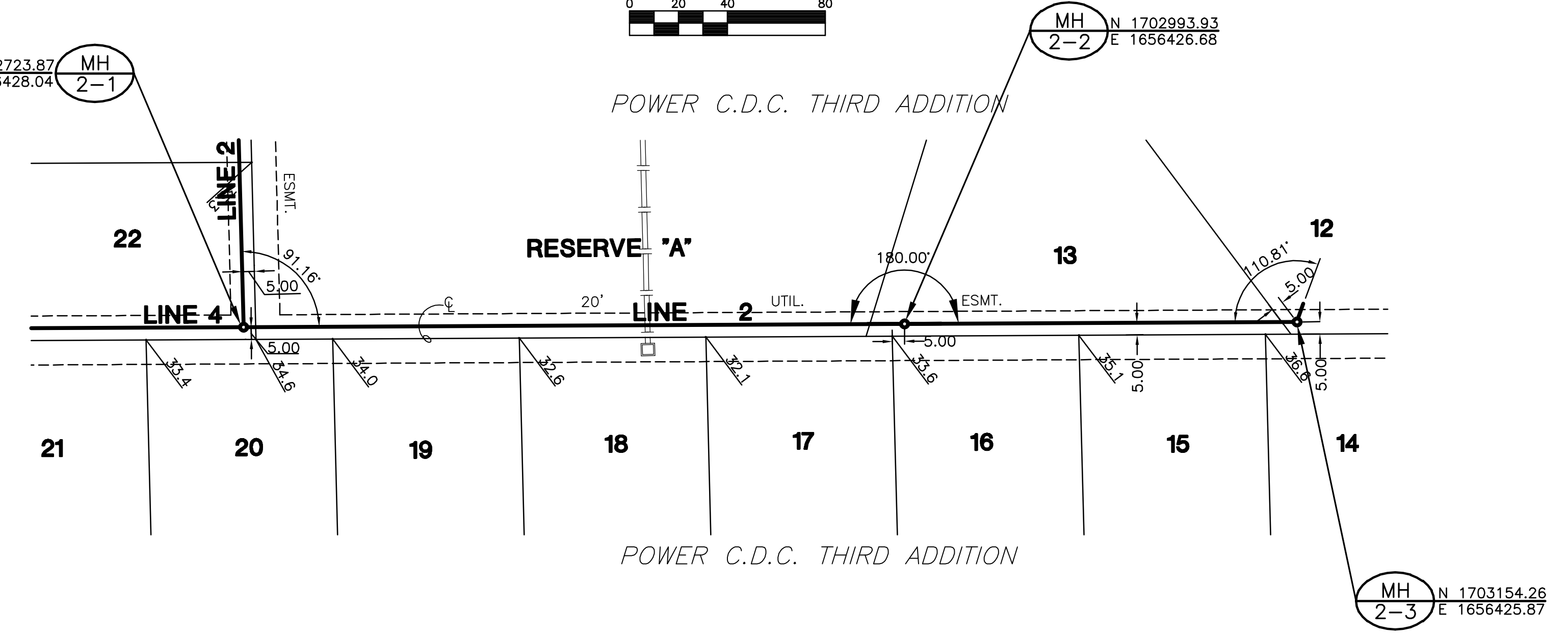
PLAN LINE 2
