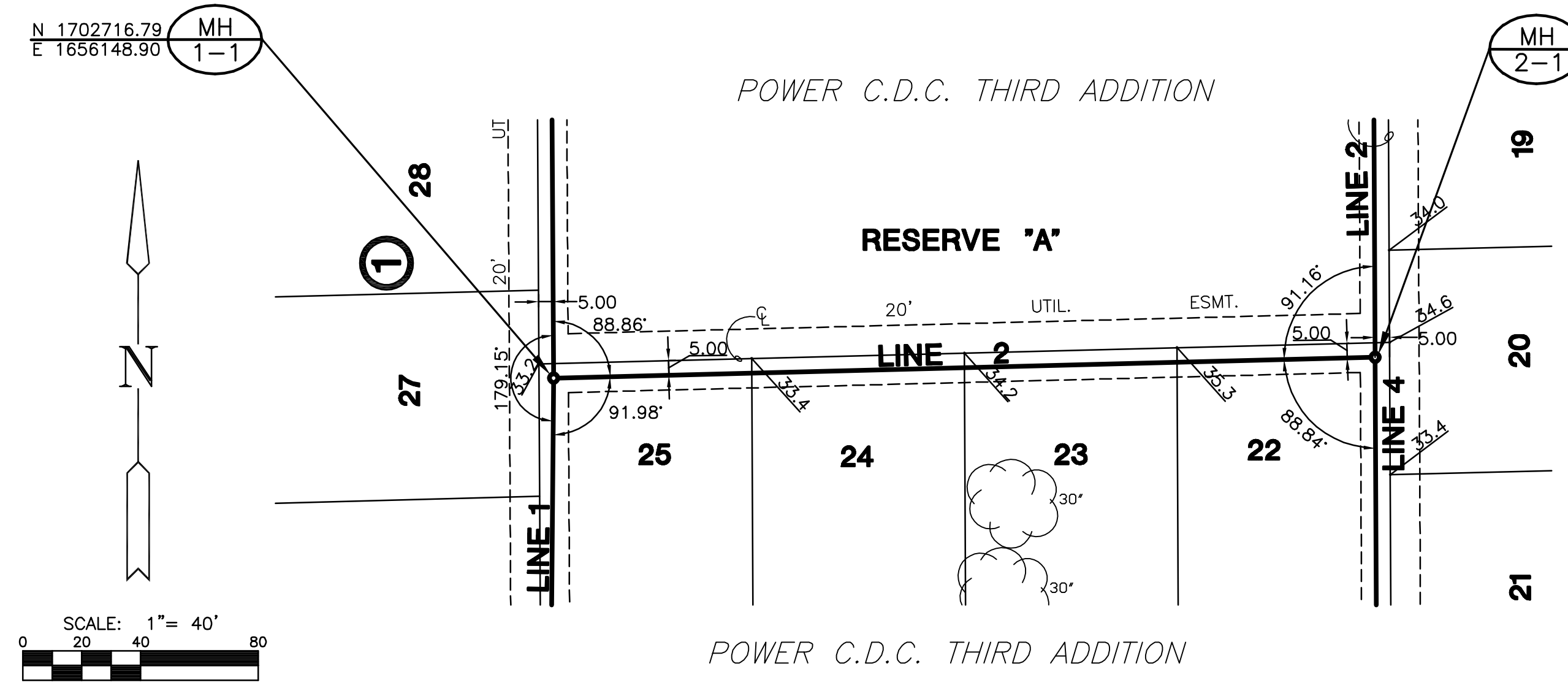
PLAN LINE 2
