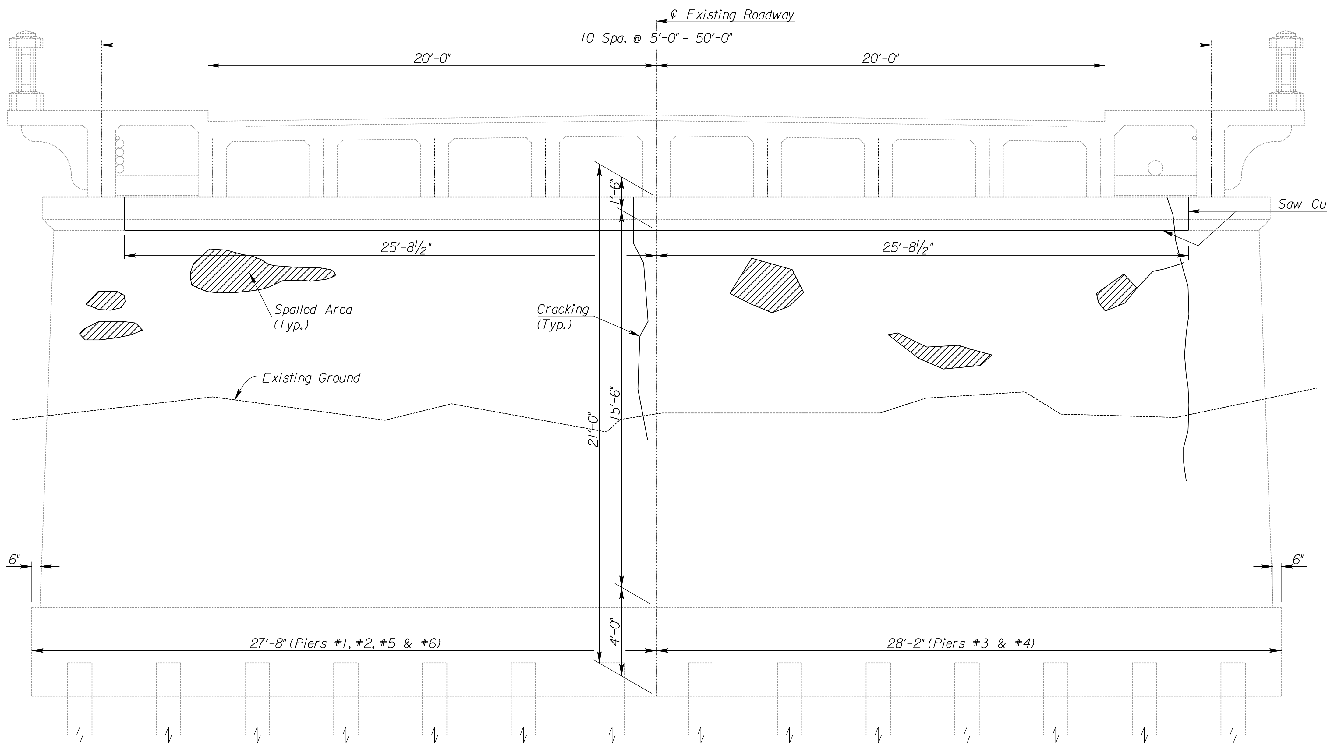
TYPICAL EXISTING PIER
