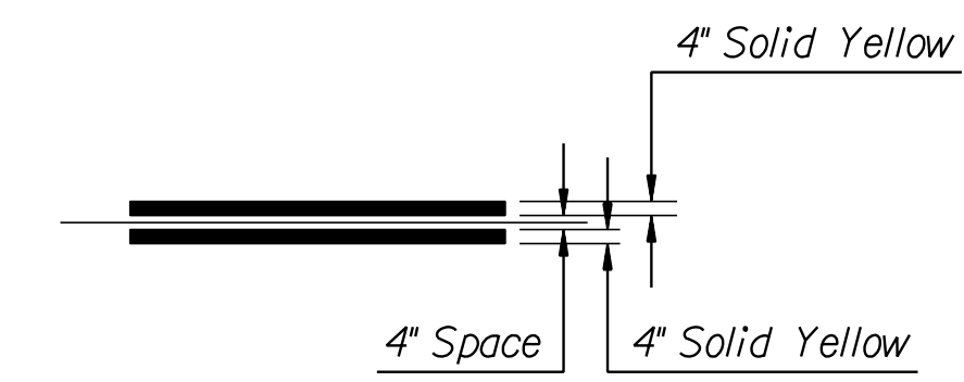
DETAIL OF DOUBLE YELLOW STRIPING
