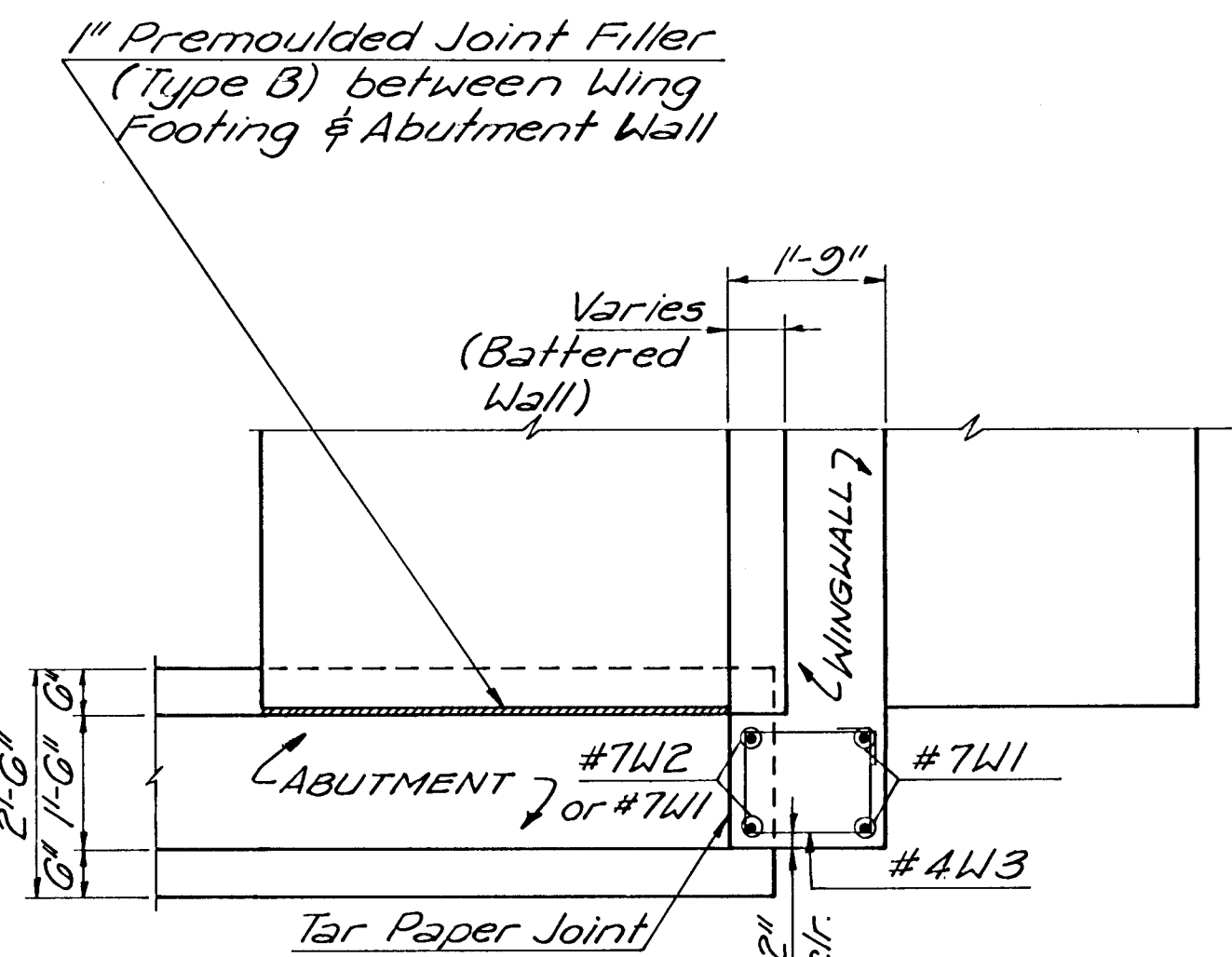
SECTION B-B
