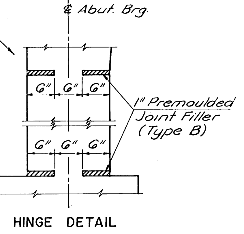
HINGE DETAIL
