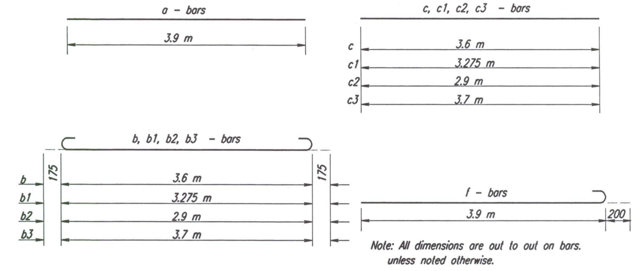
BENDING DIAGRAMS
