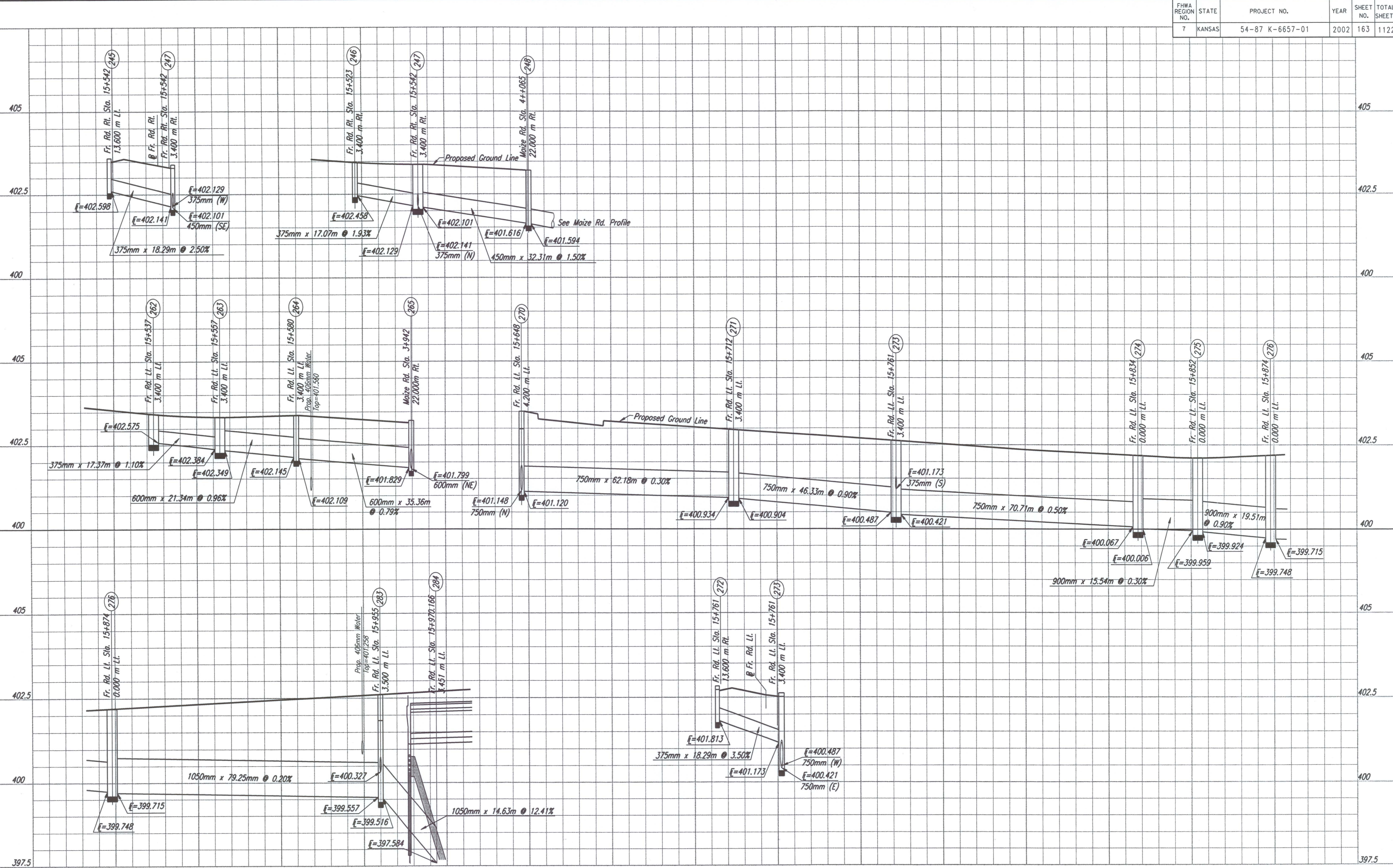
Storm Sewer Profiles Nodes 245-248, Nodes 262-265, Nodes 270-276, Nodes 283-284
