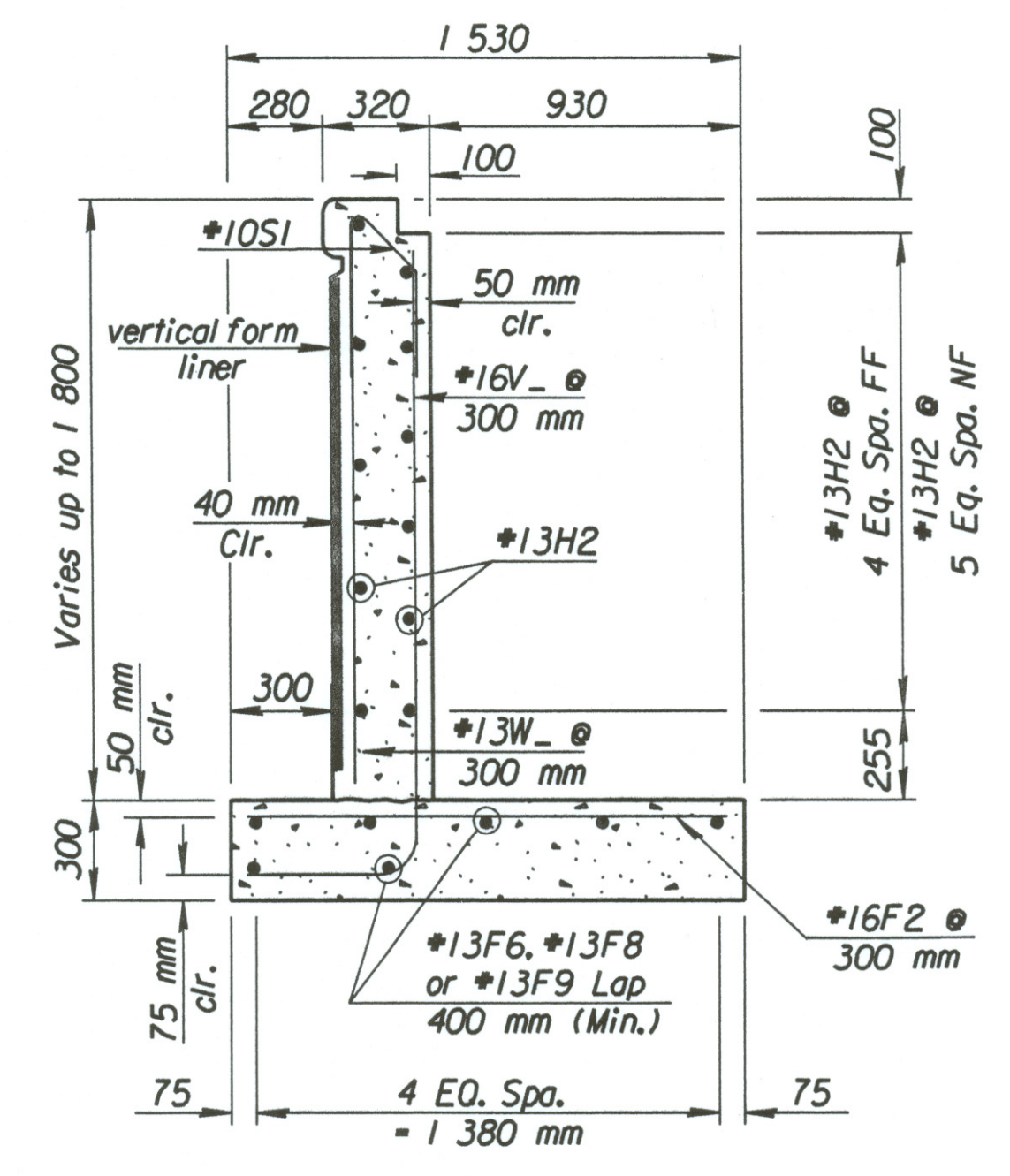
SECTION D-D (Use for Sections 4, 5, 6, 15-18, 22-25)
