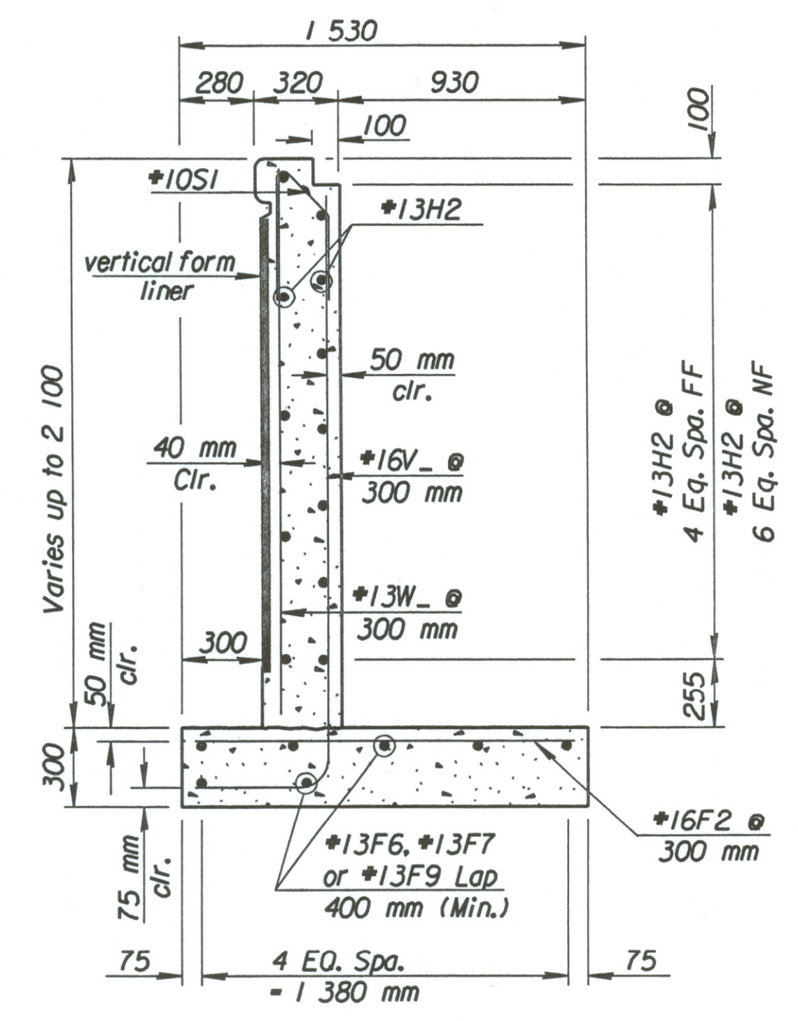
SECTION E-E (Use for Sections 7-14, 19-21)
