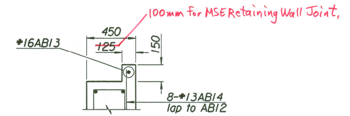
PARTIAL PLAN
