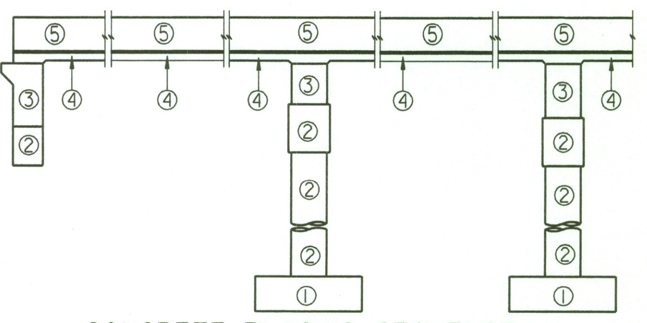
CONCRETE PLACING SEQUENCE
