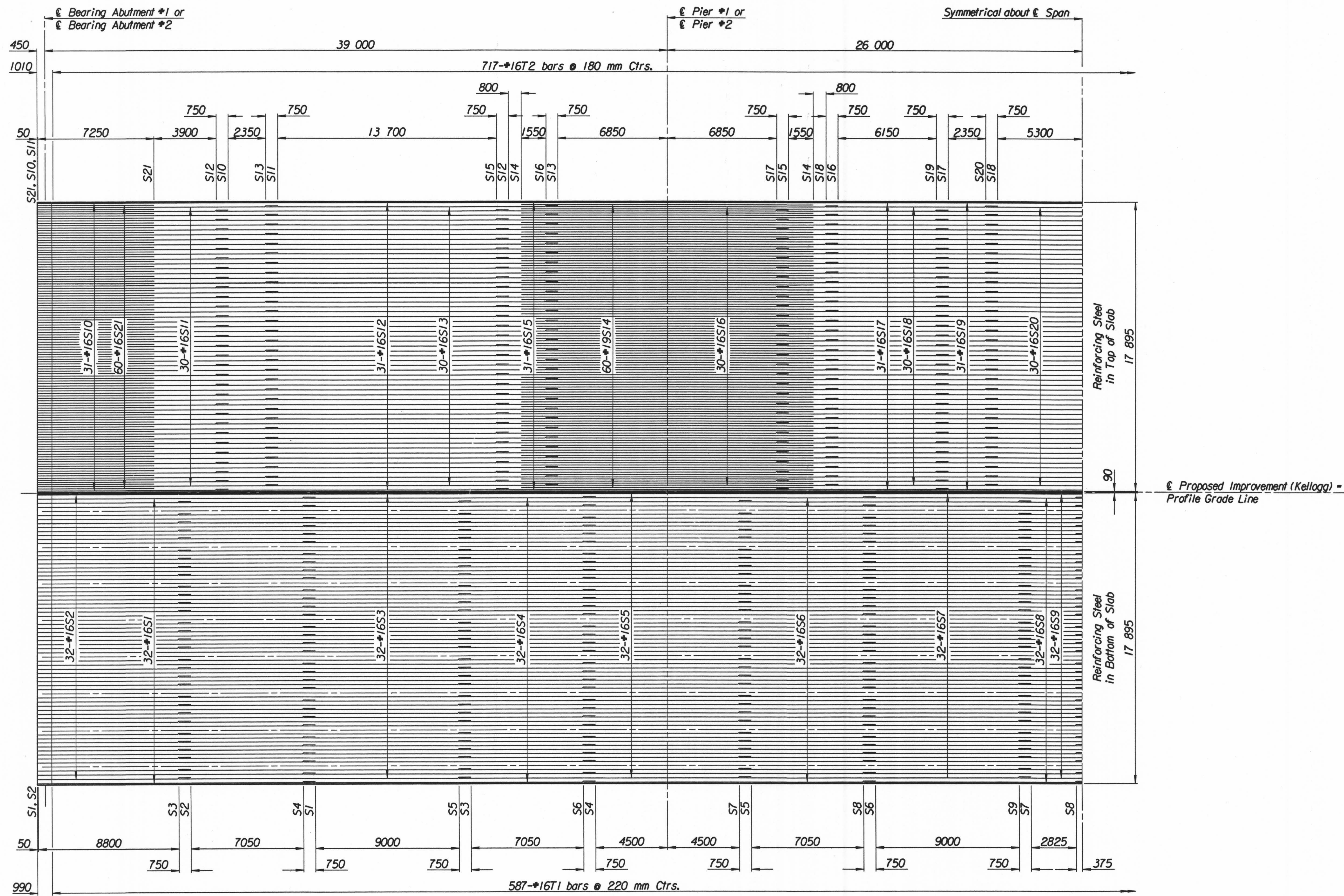
PLAN
