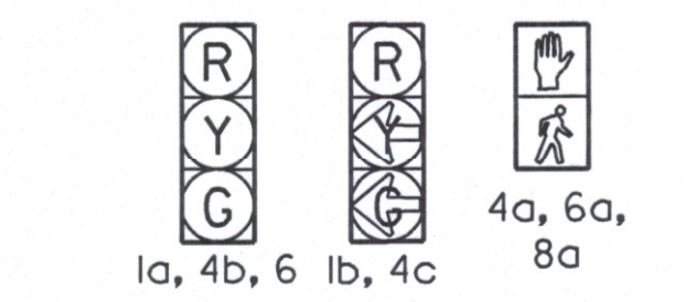
SIGNAL HEAD ARRANGMENT SOUTH INTERSECTION
