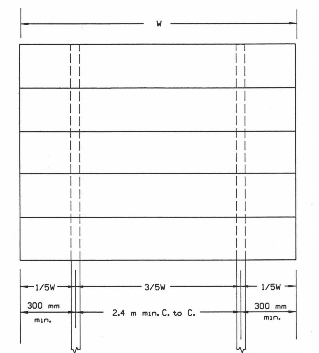
TWO POST SPACING (SEE GENERAL NOTE)
