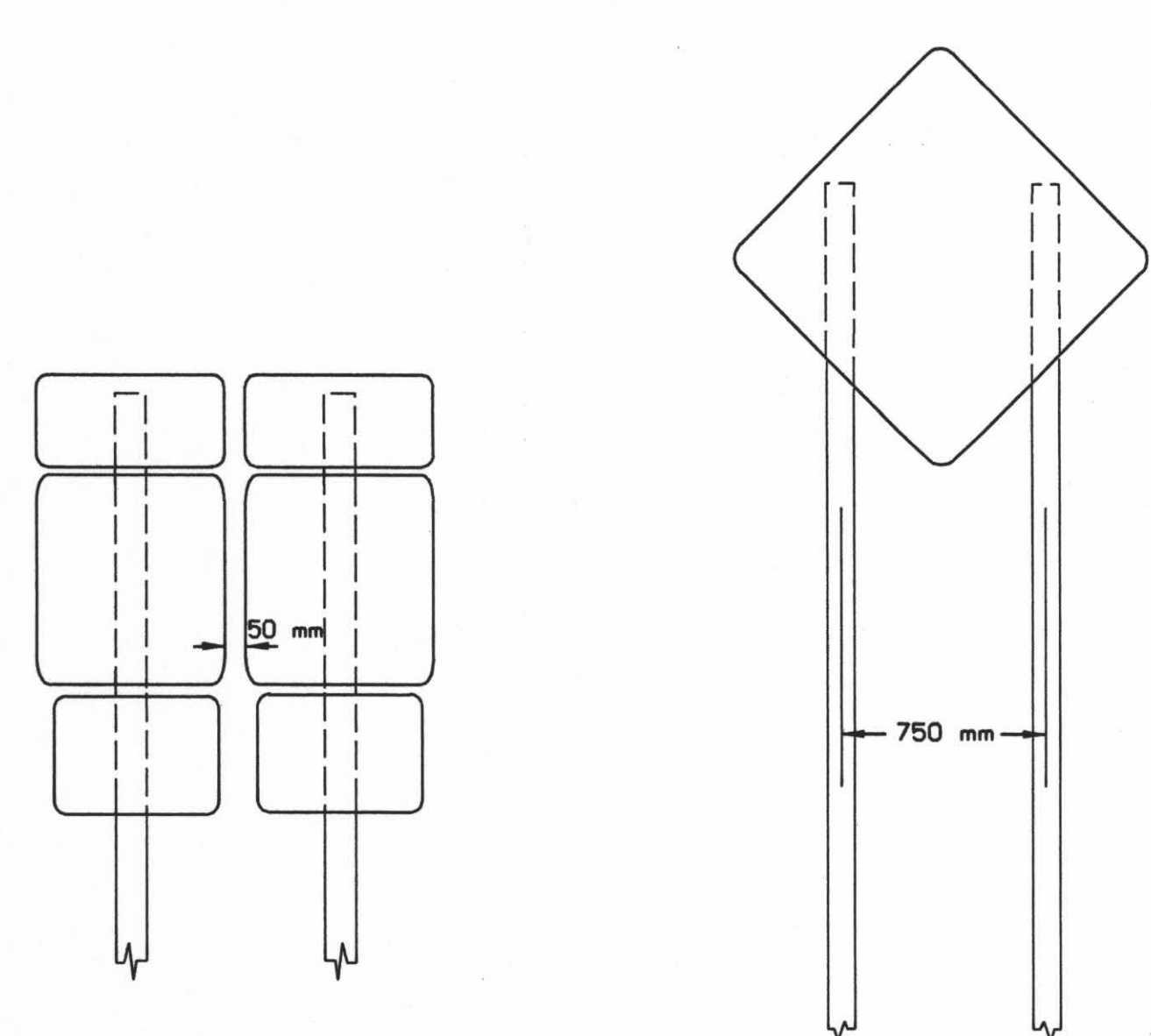
TWO POST SPACING TWO POST SPACING
