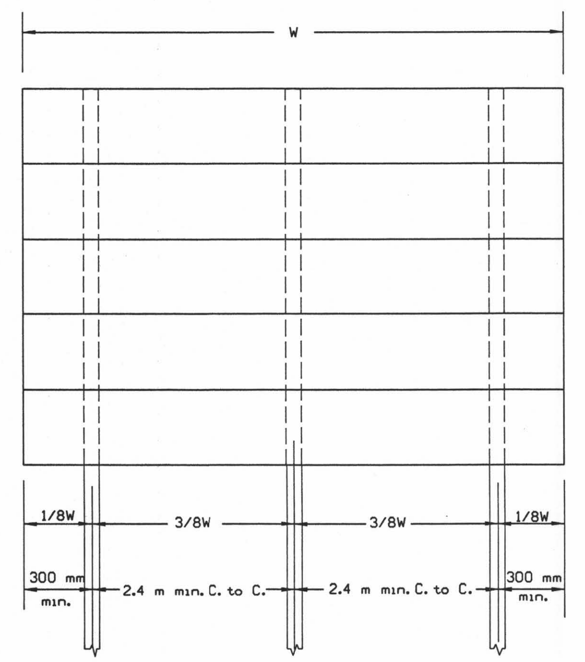
THREE POST SPACING (SEE GENERAL NOTE)
