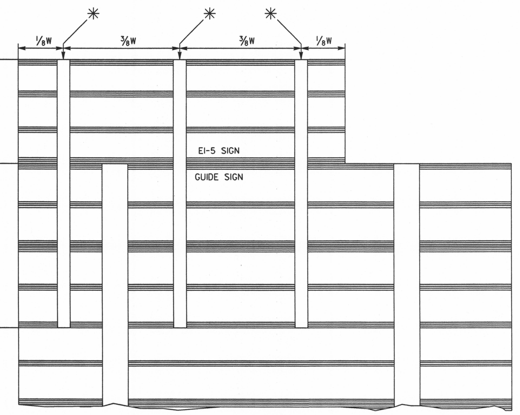
TYPICAL 3 POST MOUNTING OF EI-5 SIGN ABOVE GUIDE SIGN FOR A RIGHT EXIT
