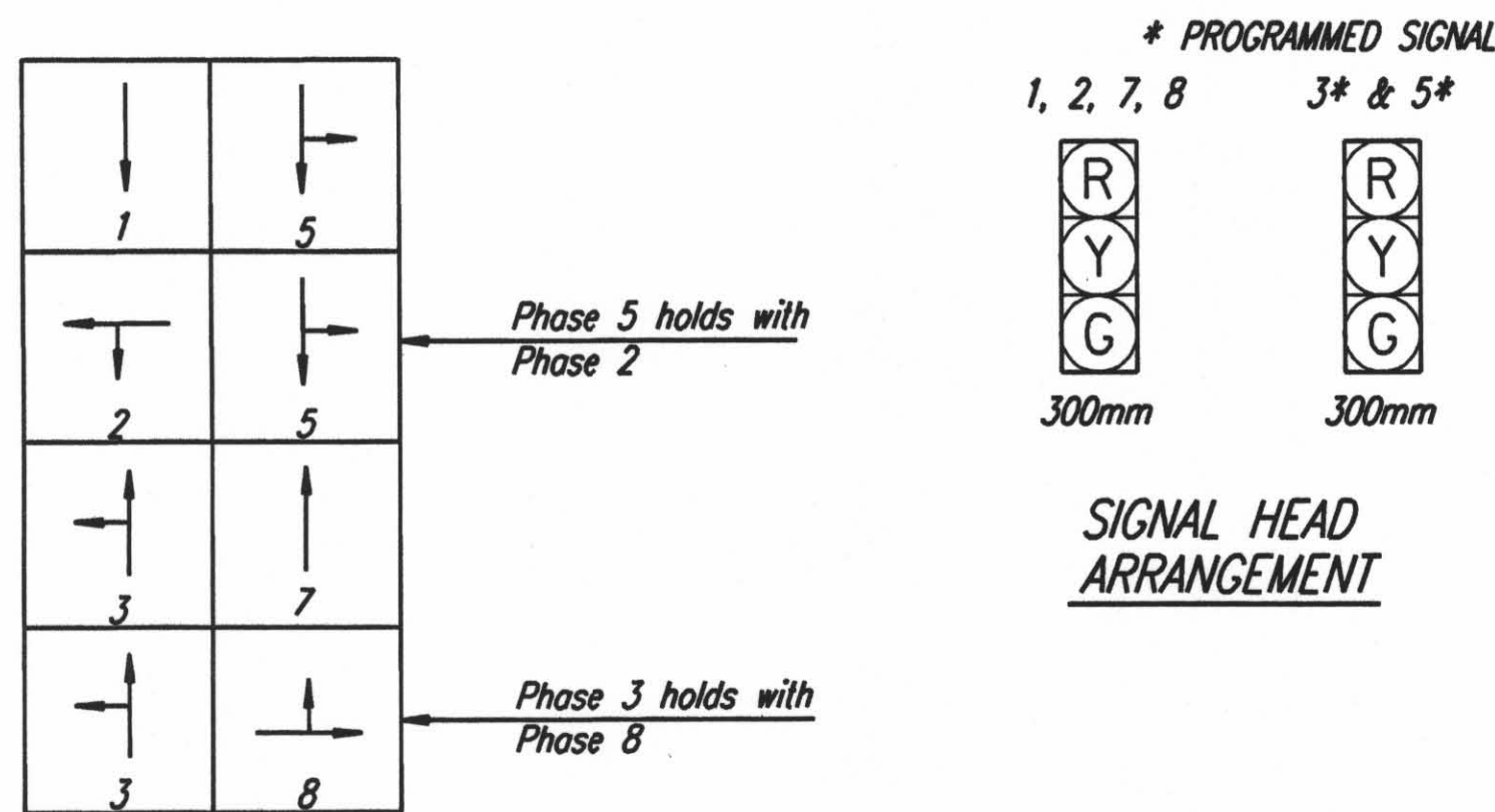
PHASE DIAGRAM STAGE 2A & 2B
