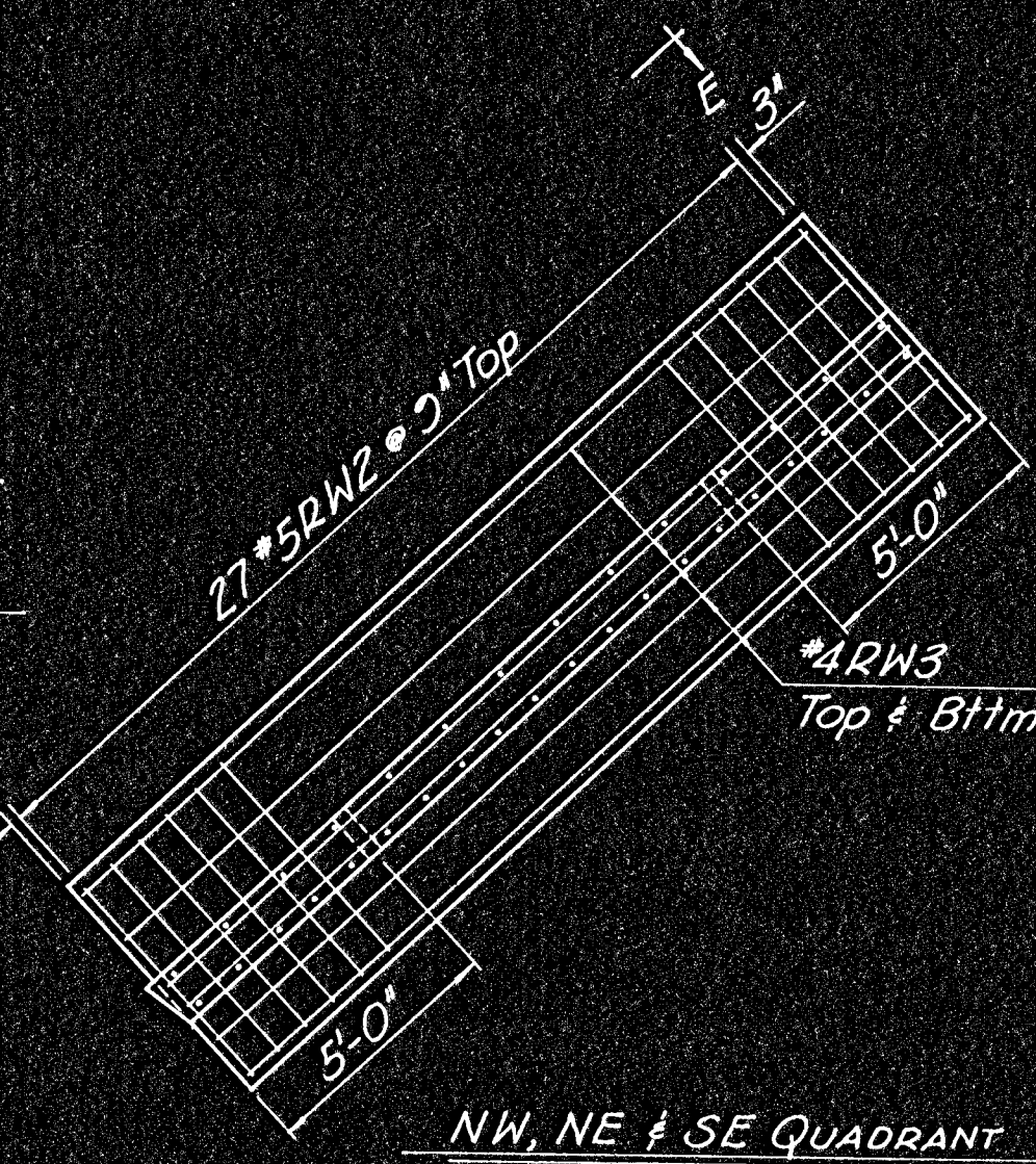
PLANS SHOWING REINFORCING
