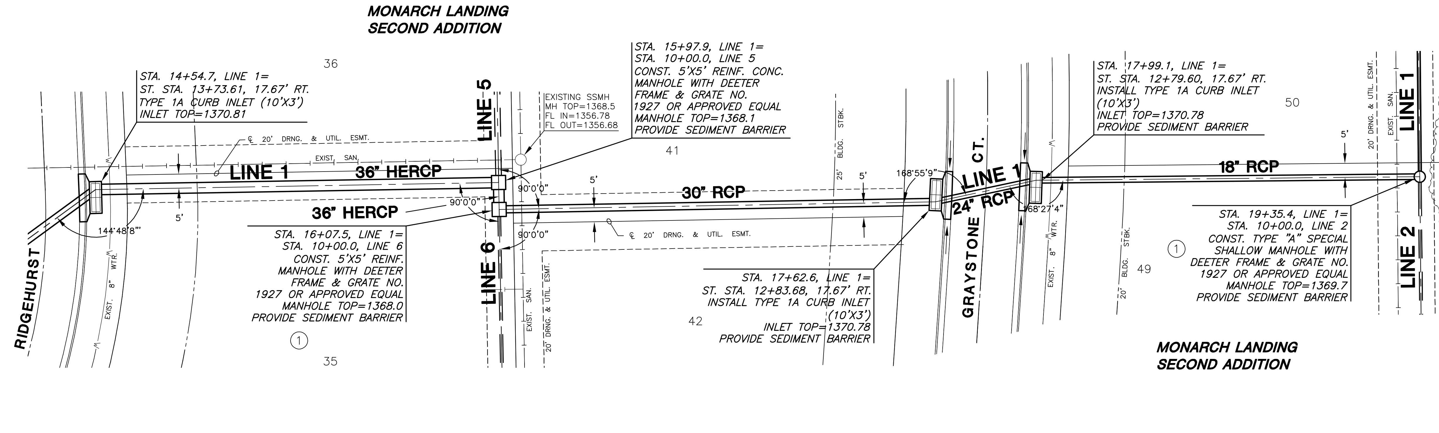
PLAN LINE 1
