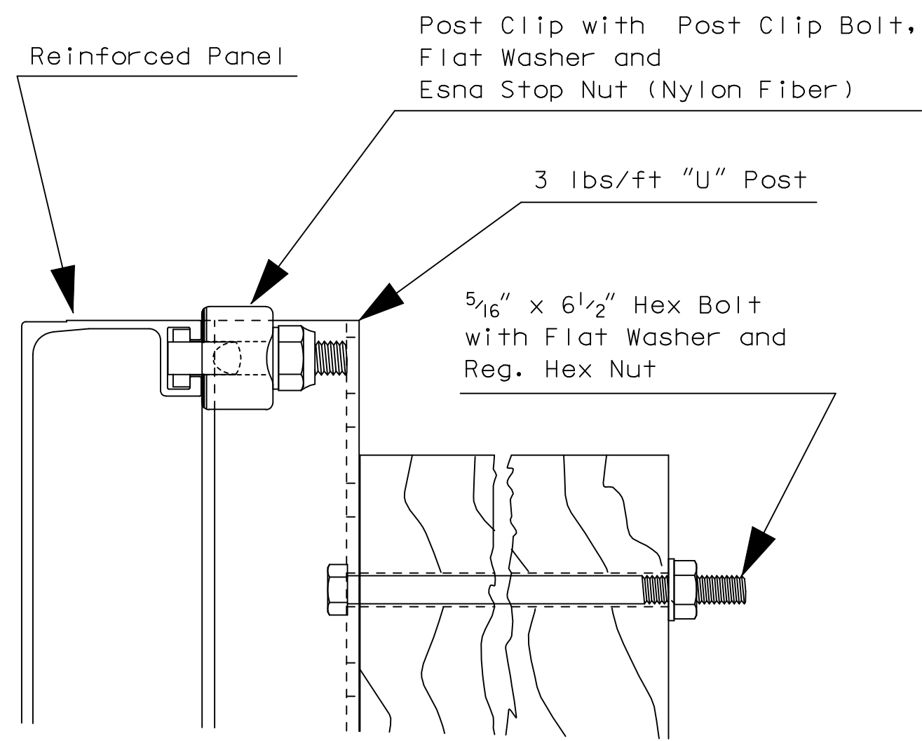
Side View
