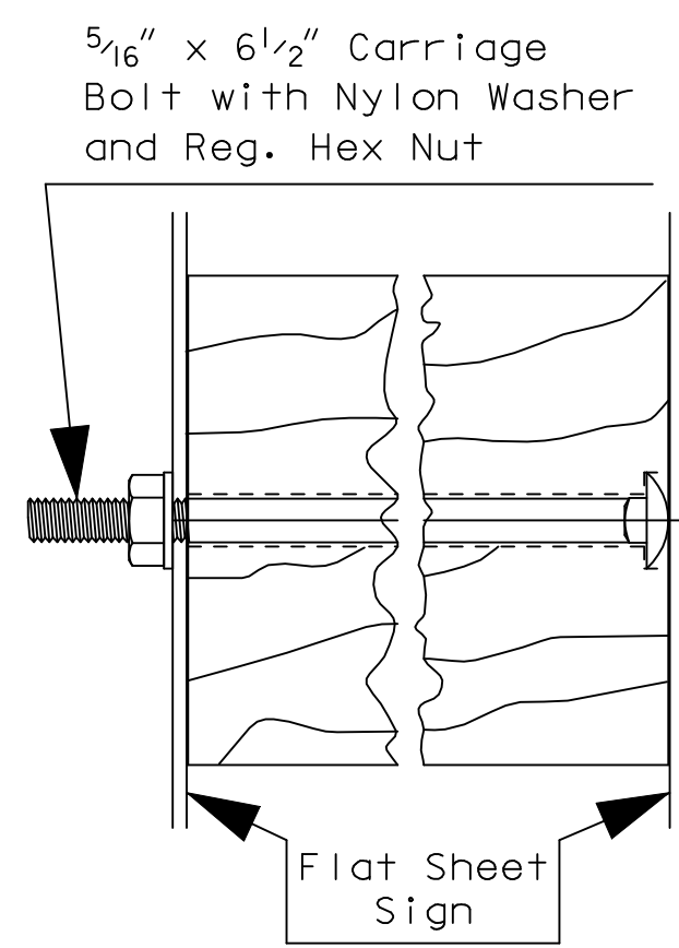
Section B-B
