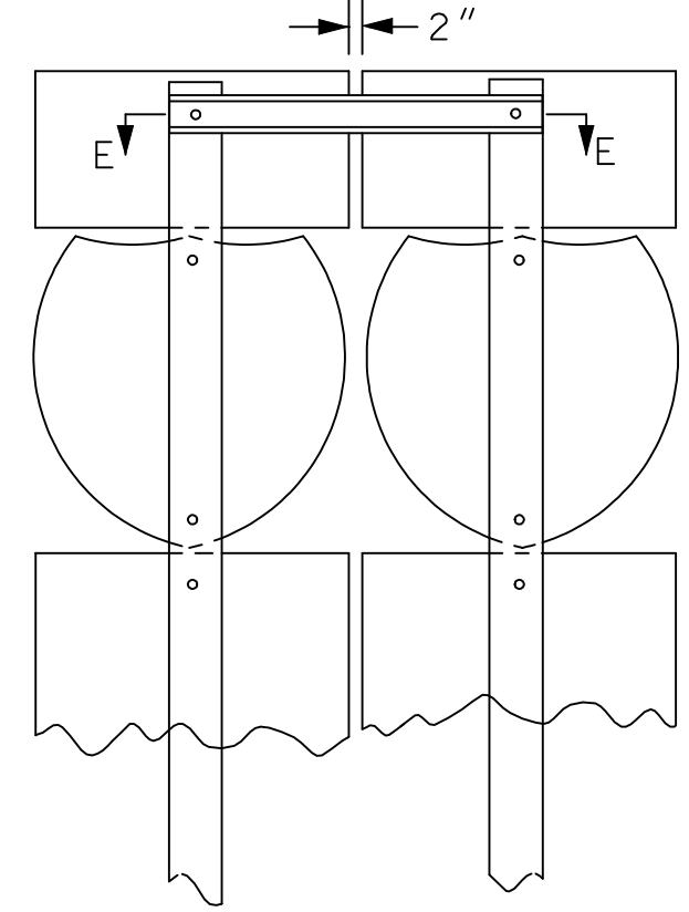
ROUTE MARKER ASSEMBLY ATTACHMENT
