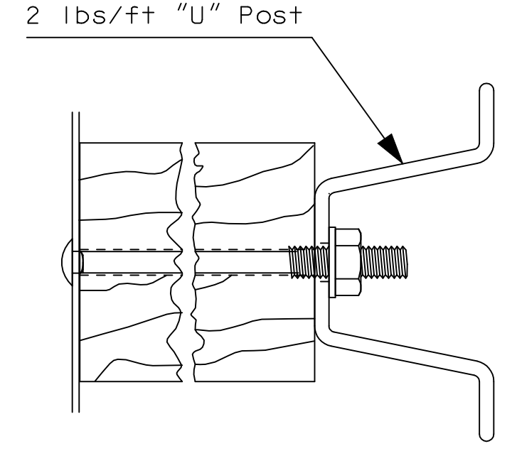
Section E-E
