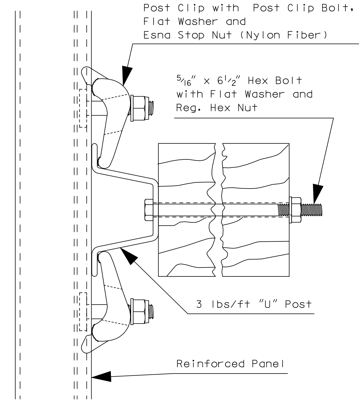
Top View
