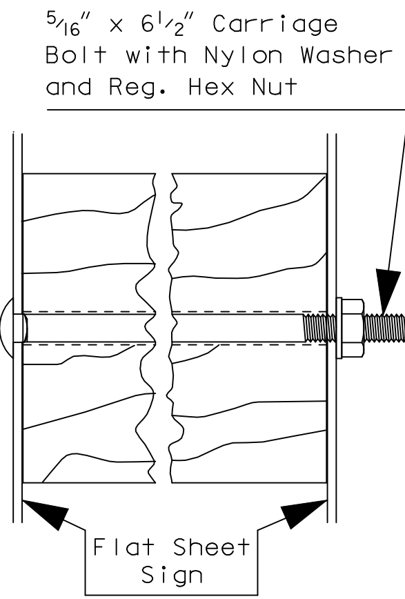
Section C-C
