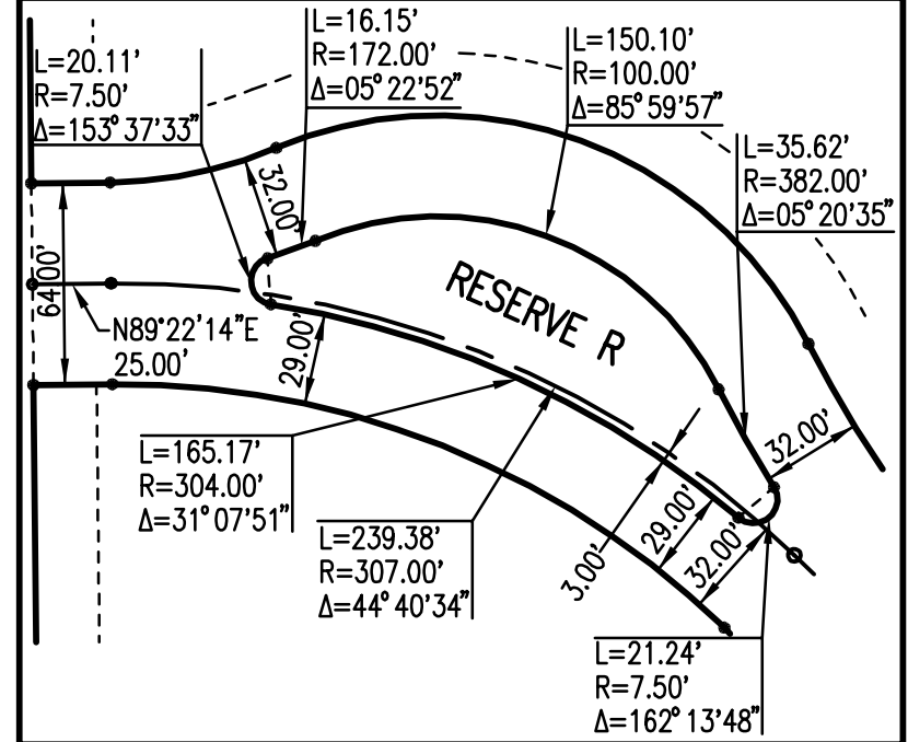
RESERVE R DETAIL
