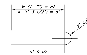
BENDING DIAGRAM
