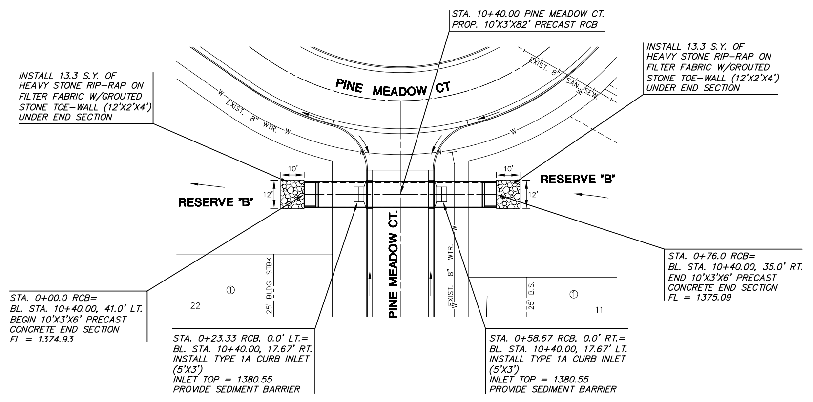
PLAN RCB SCALE: 1"=20'
