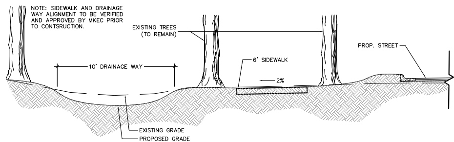
SECTION A-A NTS TYPICAL SECTION
