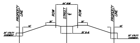
TYPICAL LOT SECTION
