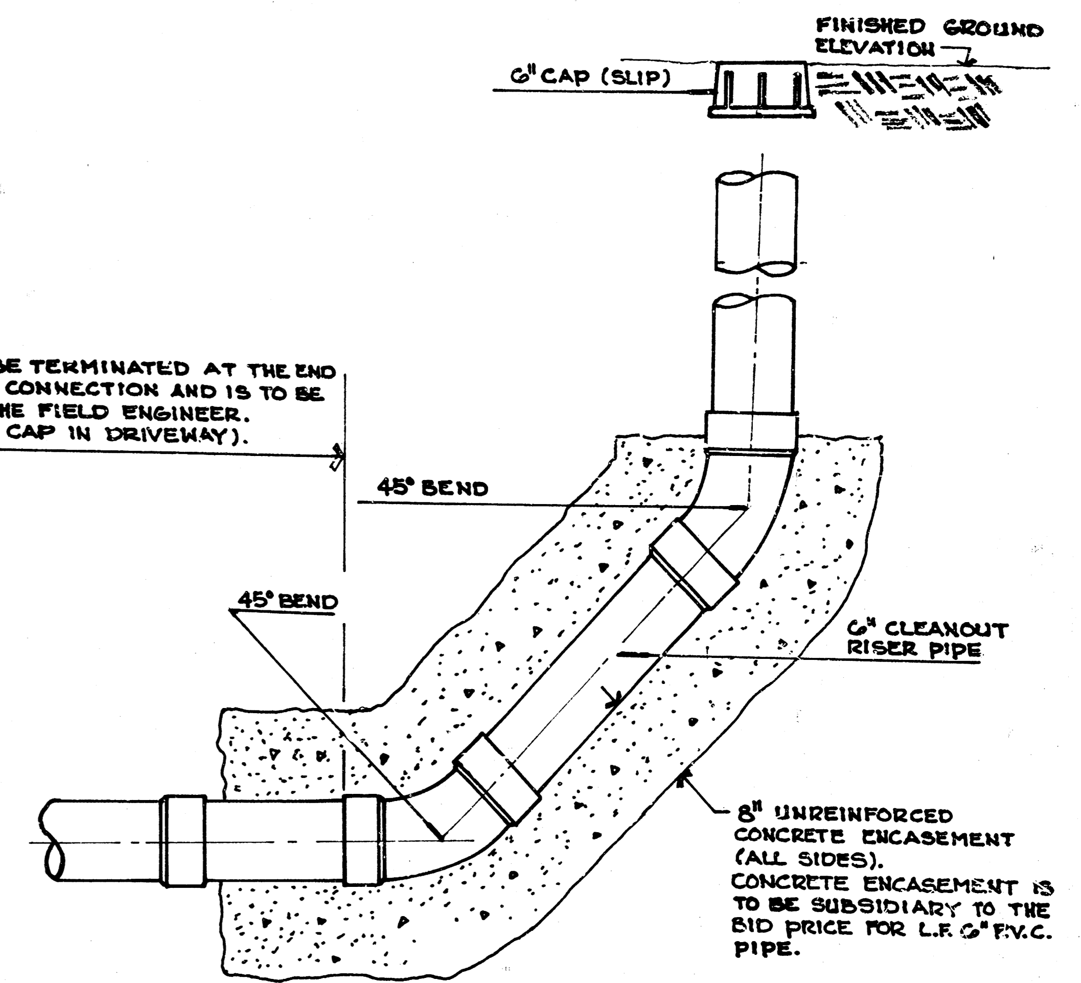
DETAIL 6" P.V.C. CLEANOUT RISER - END OF LINE-
