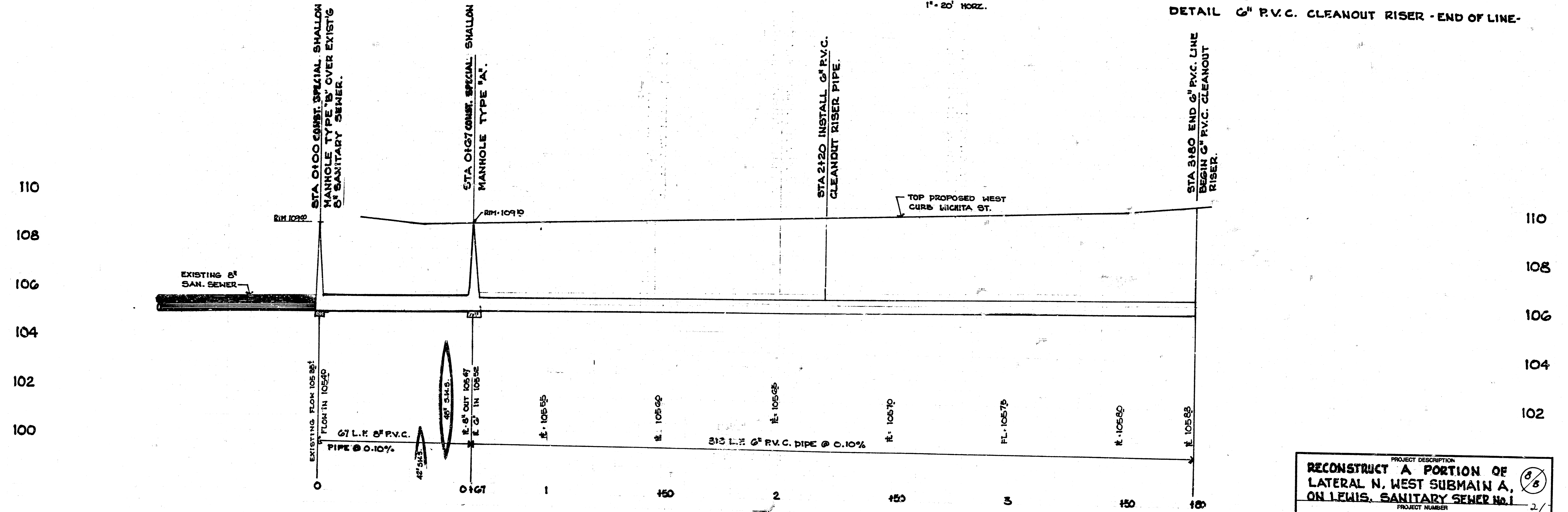
DETAIL 6" P.V.C. CLEANOUT RISER
