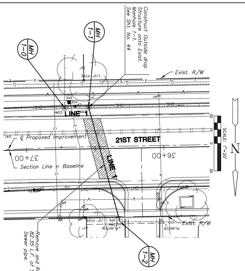
PLAN - LINE 1
