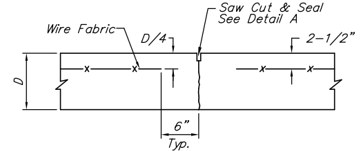
CONTRACTION JOINT DETAIL (C.J.)
