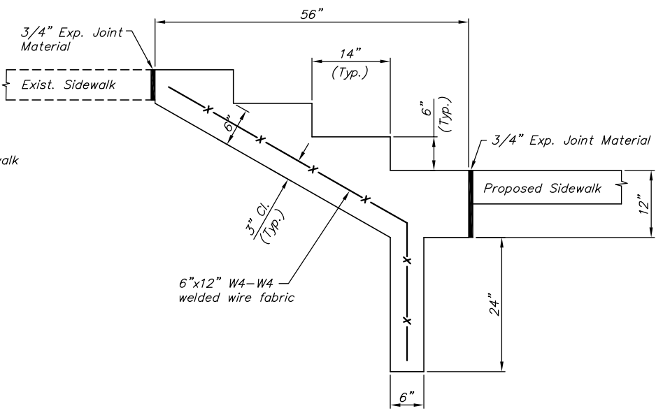
CONCRETE STEP DETAIL
