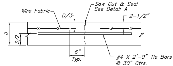
LONGITUDINAL JOINT DETAIL (L.J.)
