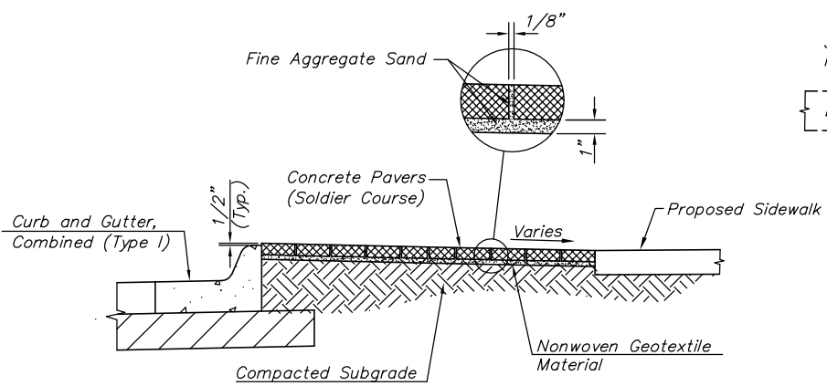
CONCRETE PAVERS DETAIL
