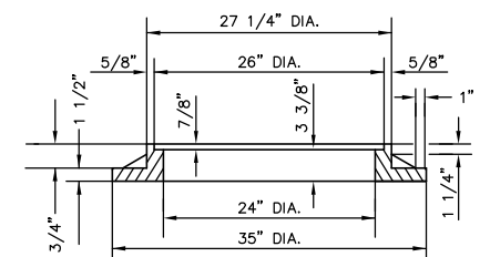
INLET FRAME
