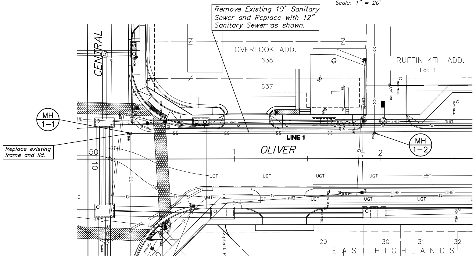
PLAN - LINE 1 SCALE: 1" = 20'
