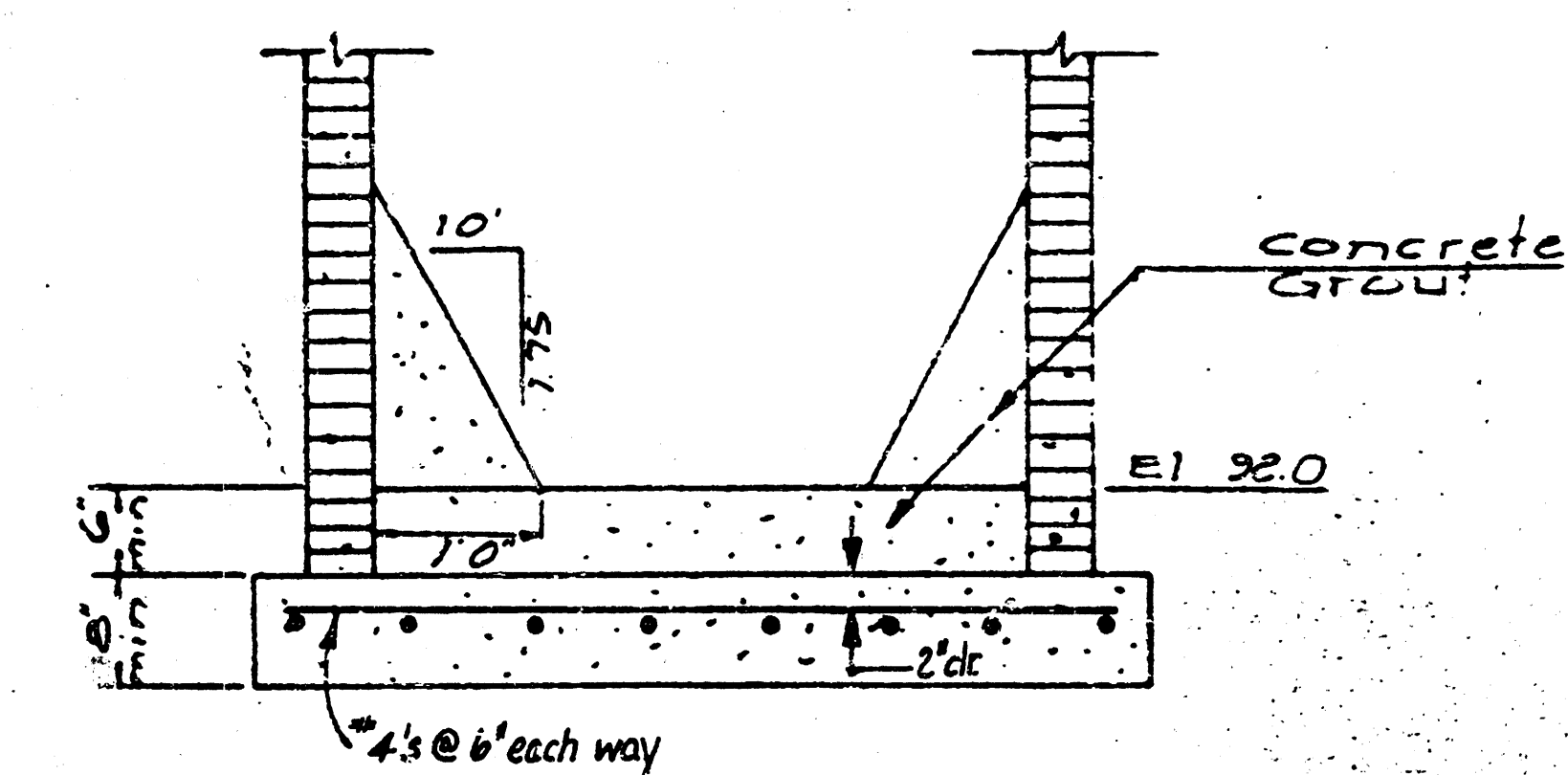
WET WELL BASE DETAIL
