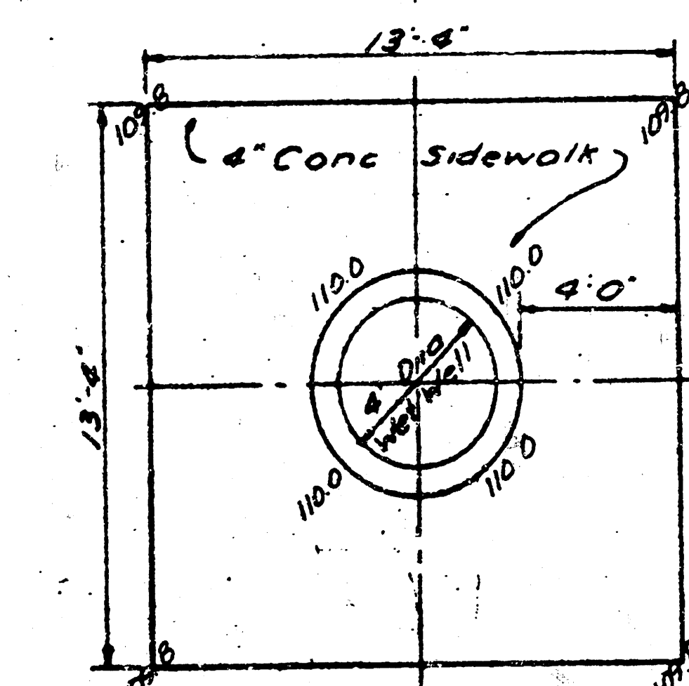
PLAN-4" PERIMETER SIDEWALK
