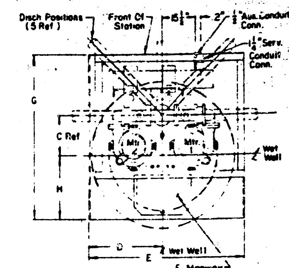
PLAN VIEW Shown Less Hood & Vent Blower
