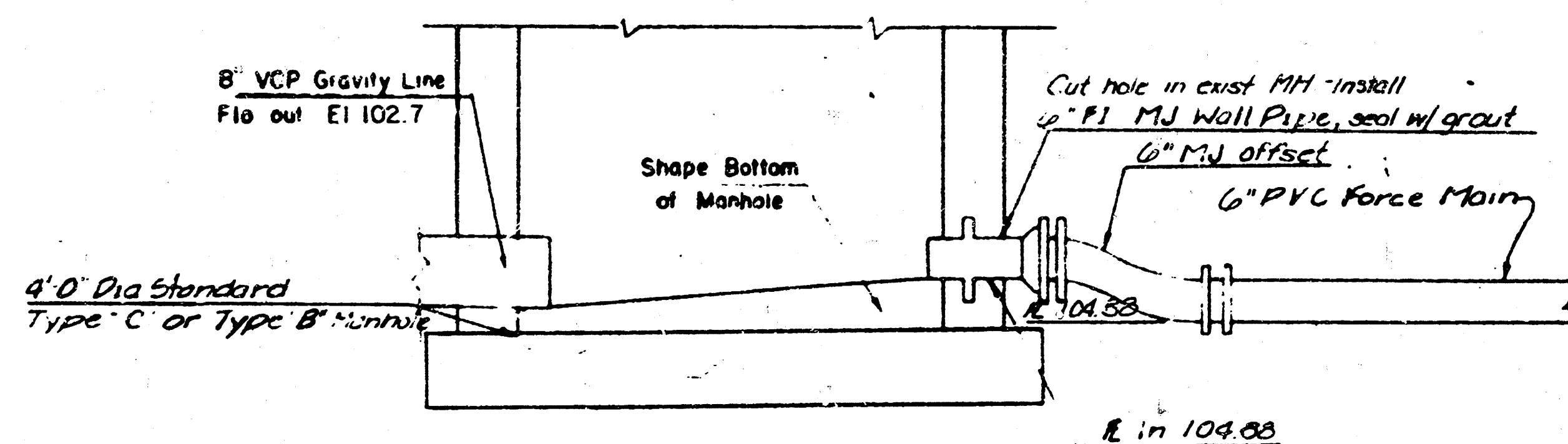
STANDARD MANHOLE WITH FORCE MAIN CONNECTION
