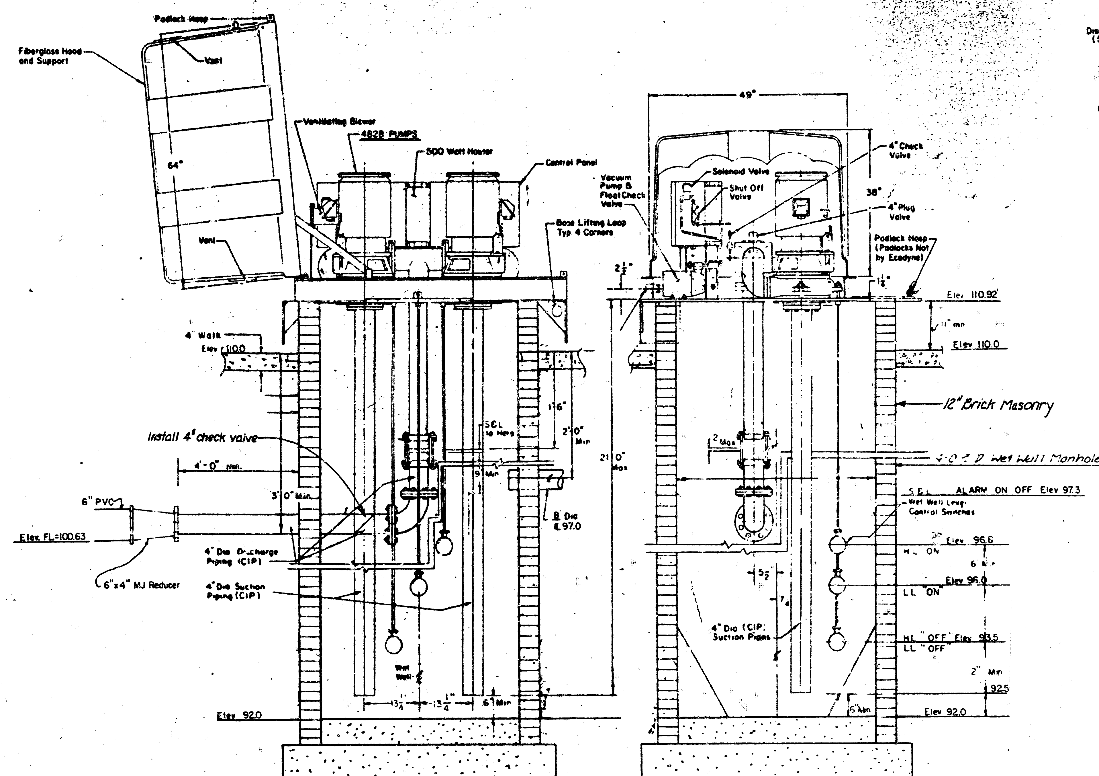
SMITH & LOVELESS LIFT STATION
