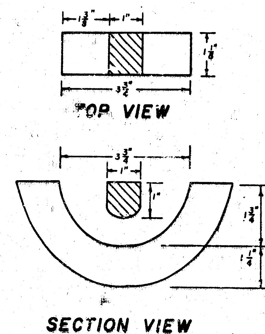
SECTION VIEW
