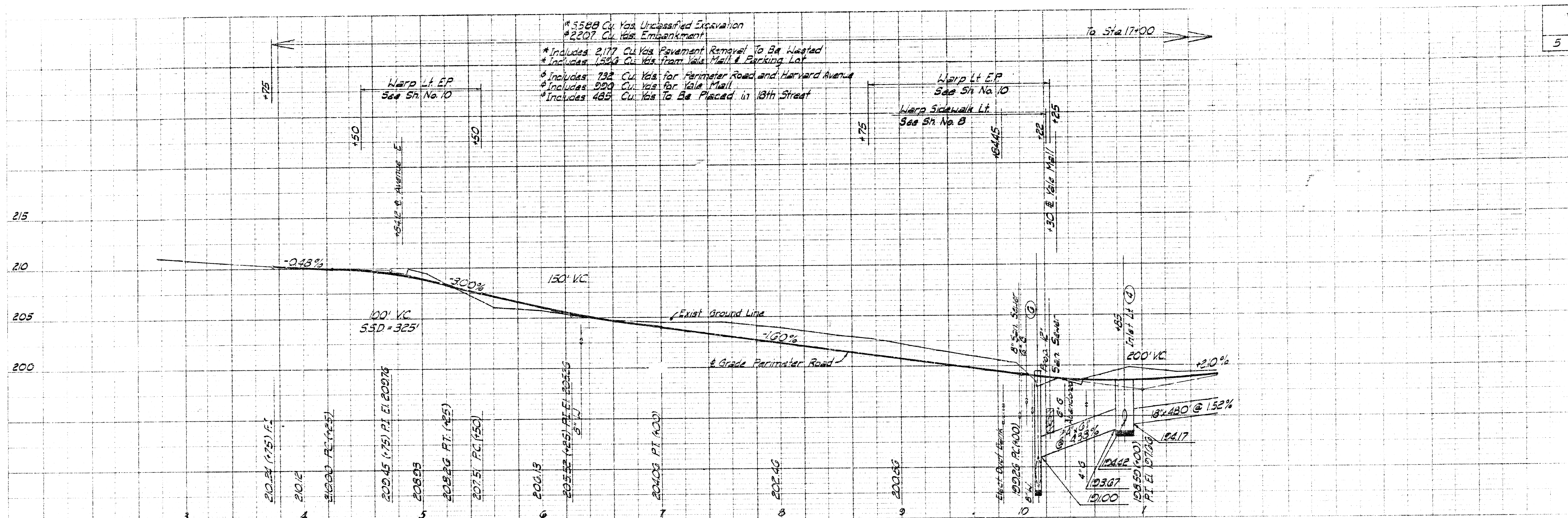
PERIMETER ROAD SECTION 2
