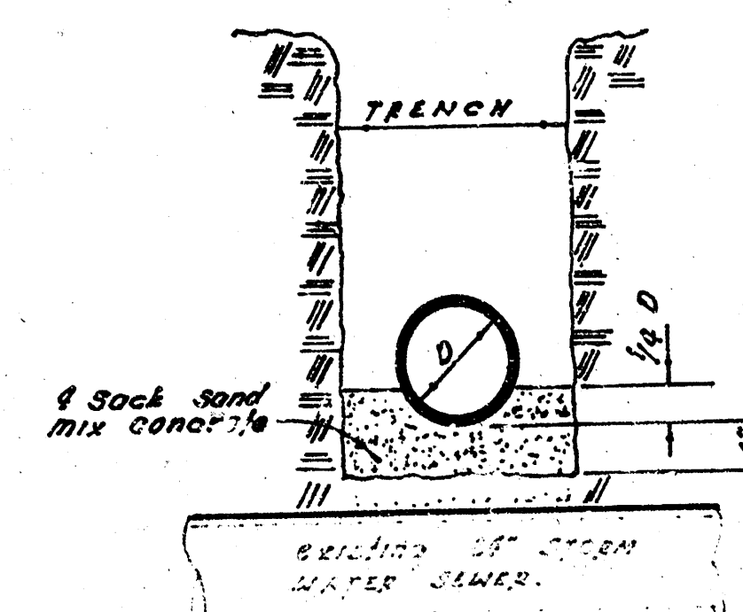
DETAIL CONCRETE CRADLE in Sack
