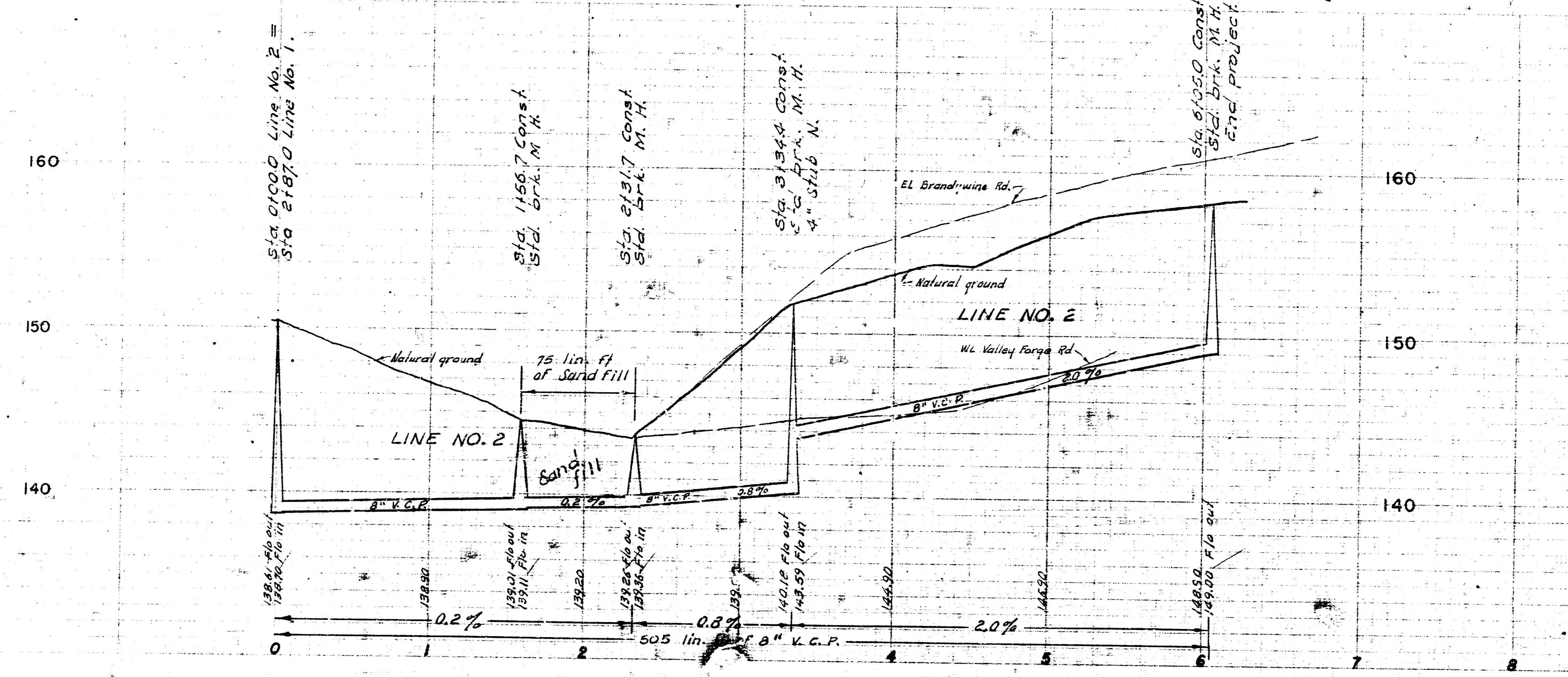
B. M. 151.08 BRIDGE SPIKE W. SIDE P.P. FIRST S. OF BRANDYWINE & E. OF VALLEY FORGE RD.
