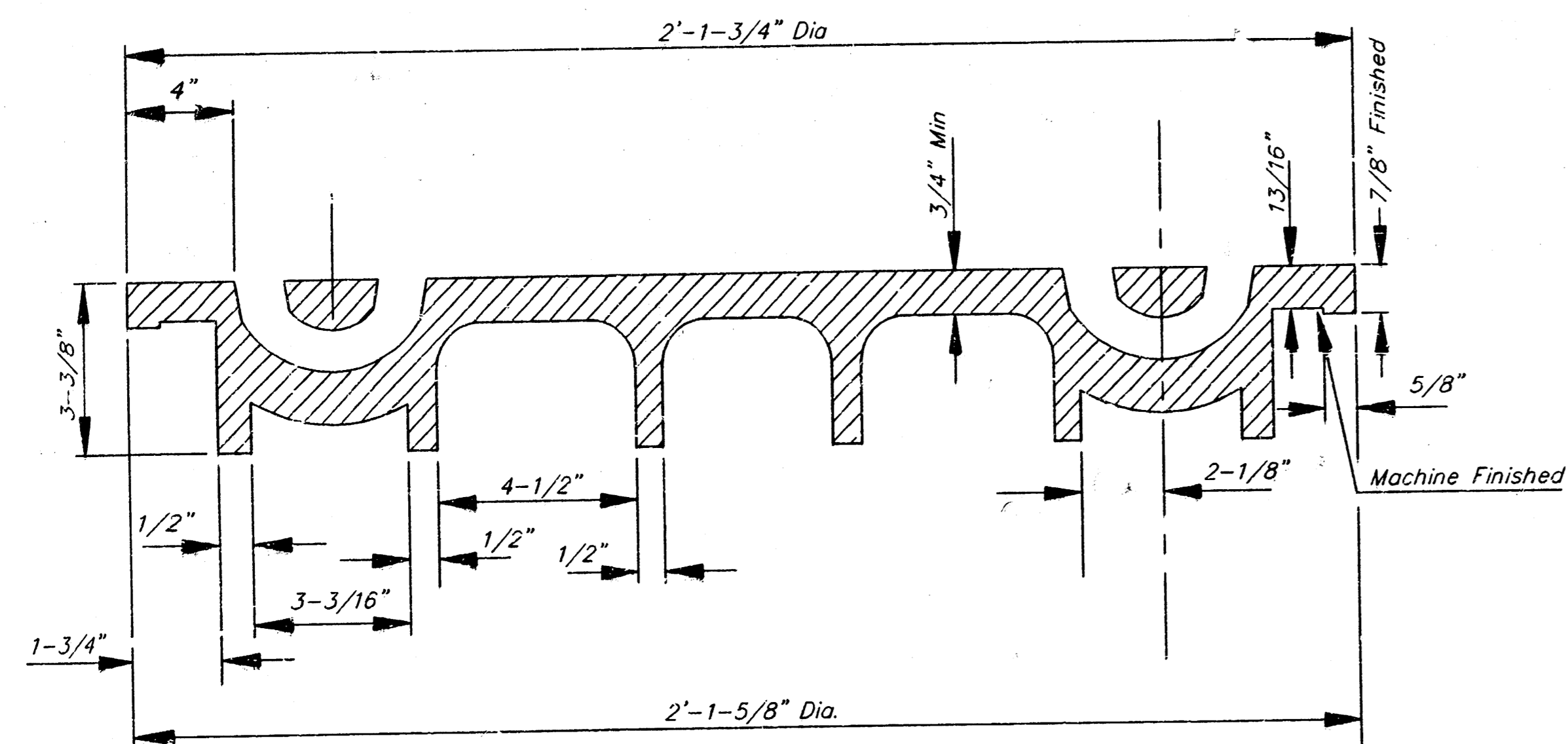
SECTION VIEW
