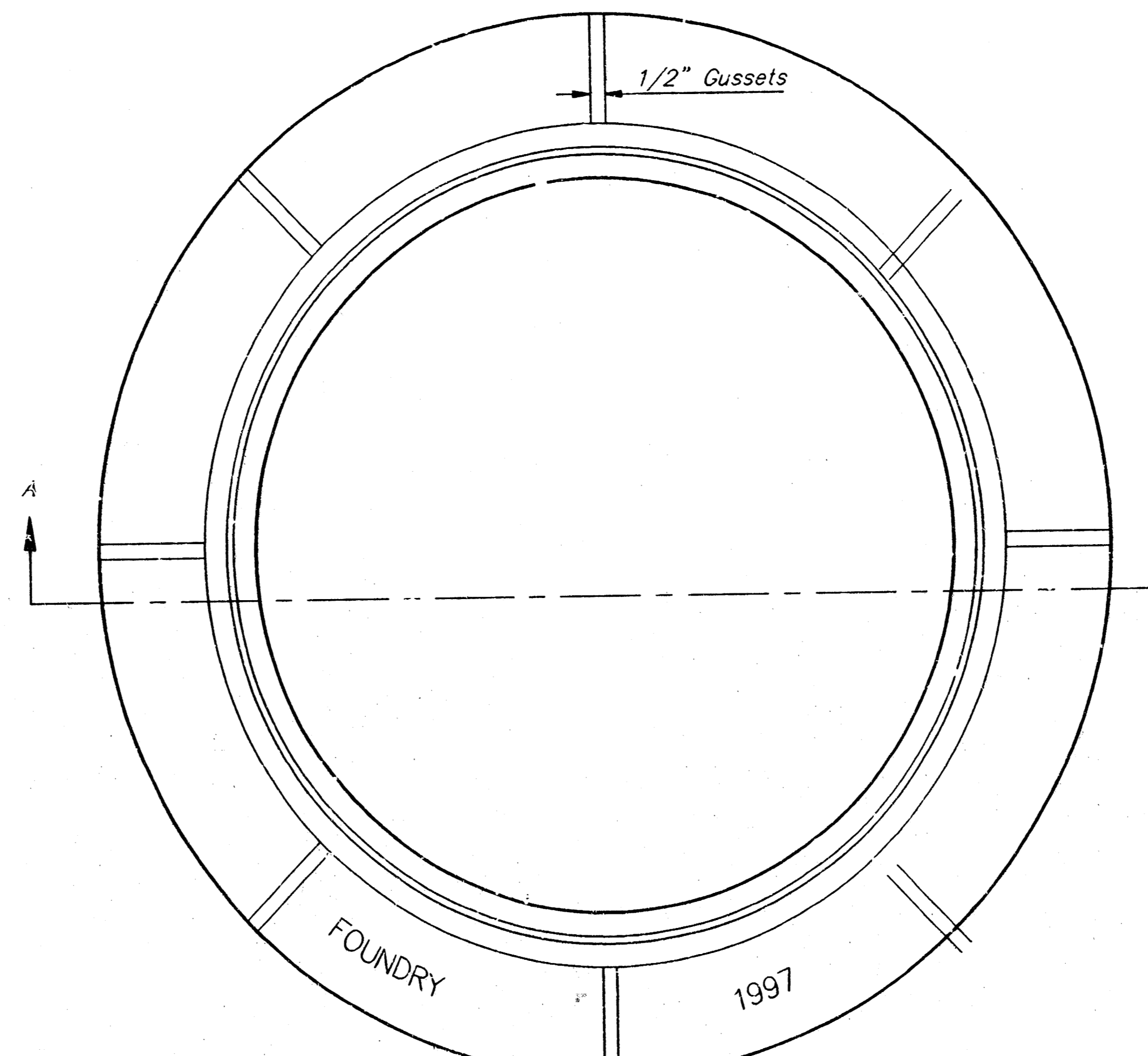
TOP VIEW
