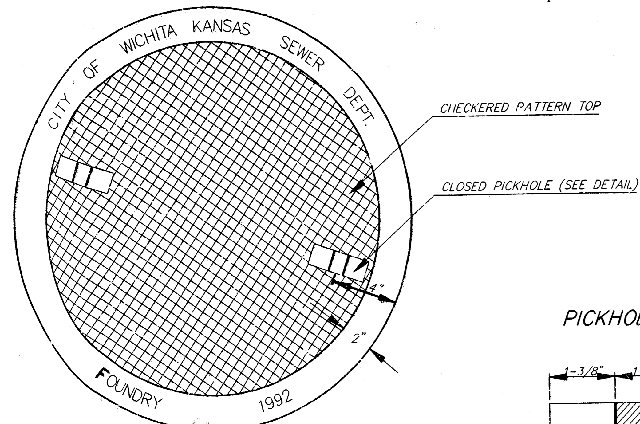
TOP VIEW
