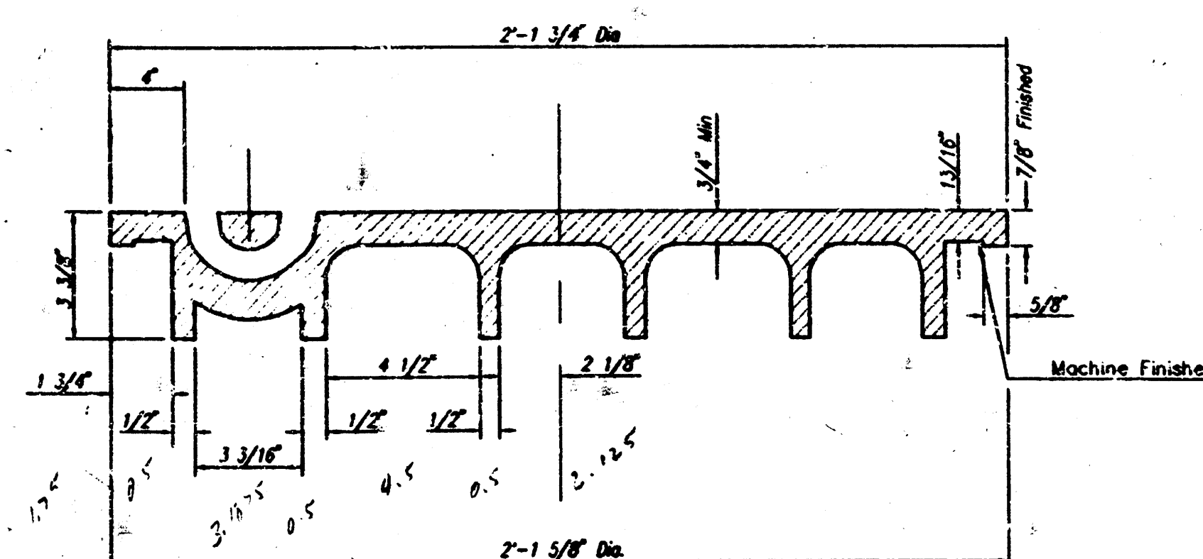
SECTION VIEW
