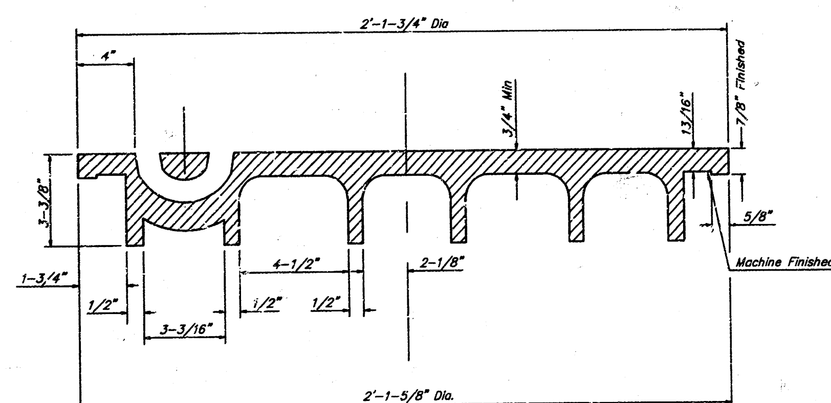
SECTION VIEW
