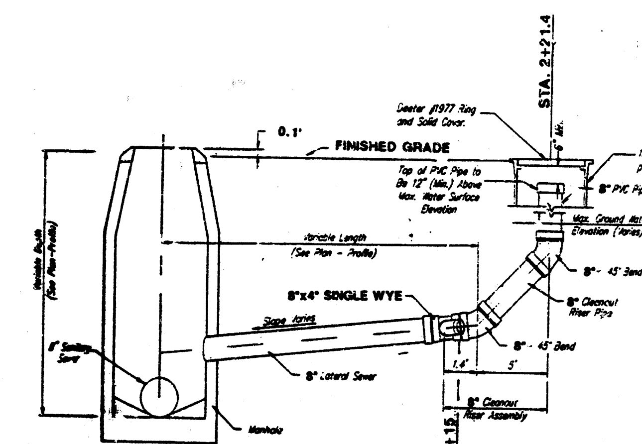
8" CLEANOUT RISER ASSEMBLY DETAIL
