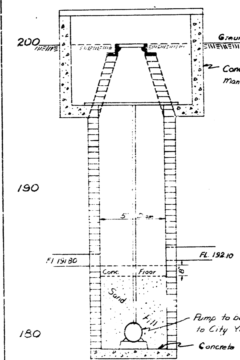
DETAILS FOR REMODELING MANHOLE 30+46
